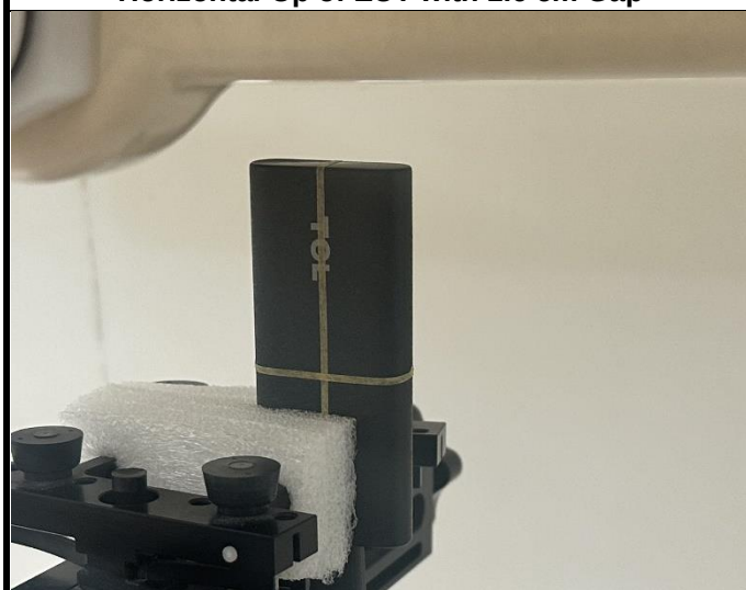
Vertical-Top of EUT with 1.6 cm Gap
