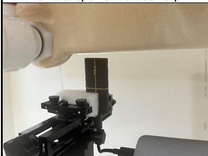
Vertical-Top of EUT with 0.5 cm Gap
