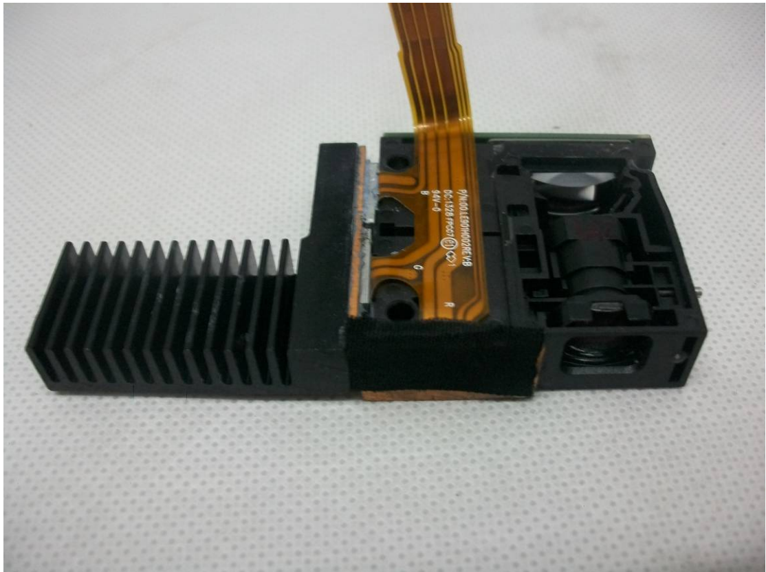
INTERNAL PHOTO OF SAMPLE -8
