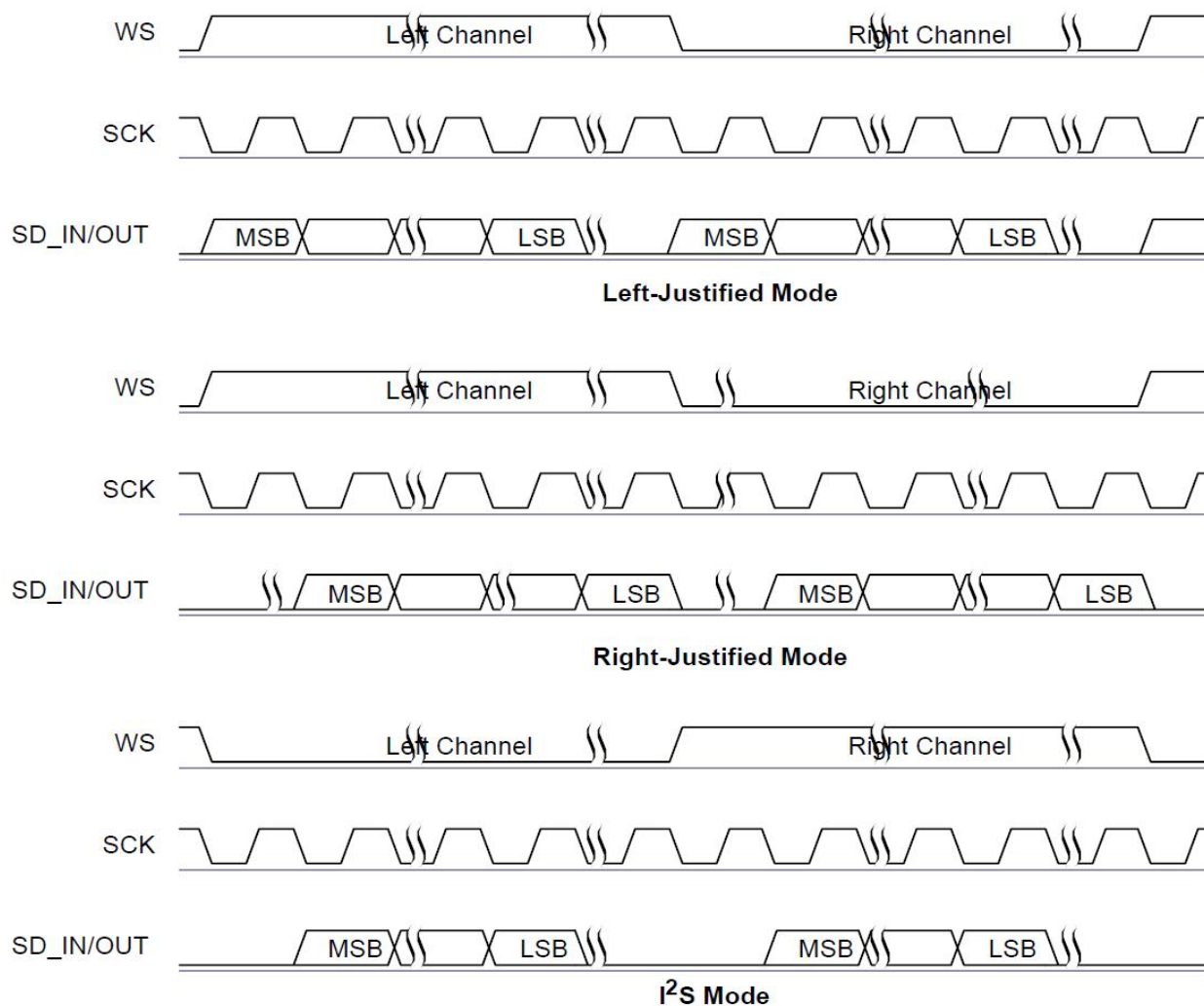
Figure 5 : Digital Audio Interface Modes
