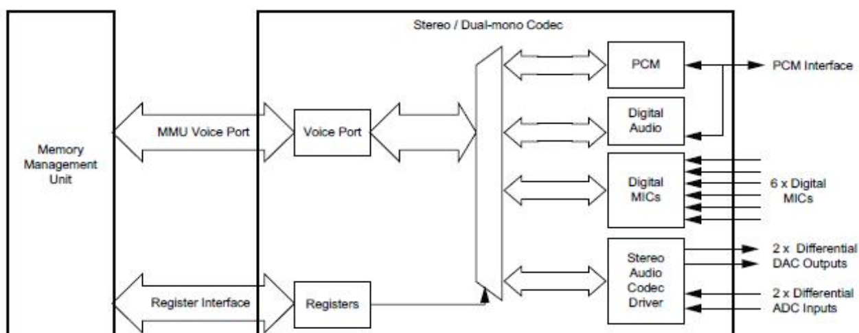
Figure 4 : Audio Interface
