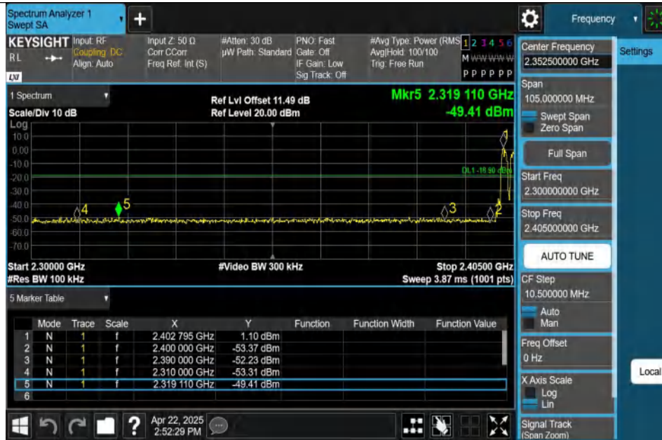
3DH5-Ant1-Hop_2402-PASS
