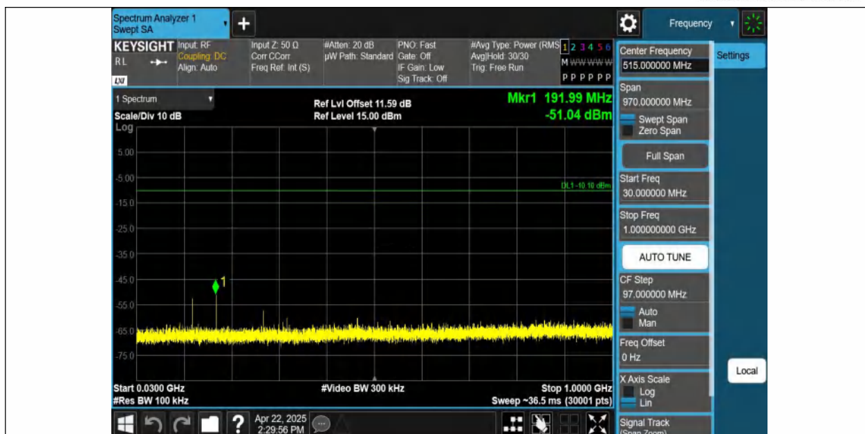
2DH5-Ant1-2480-30~1000-PASS
