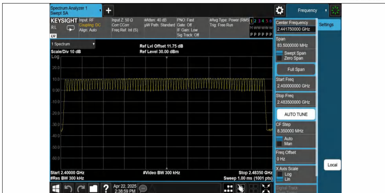
DH5-Ant1-Hop-PASS
