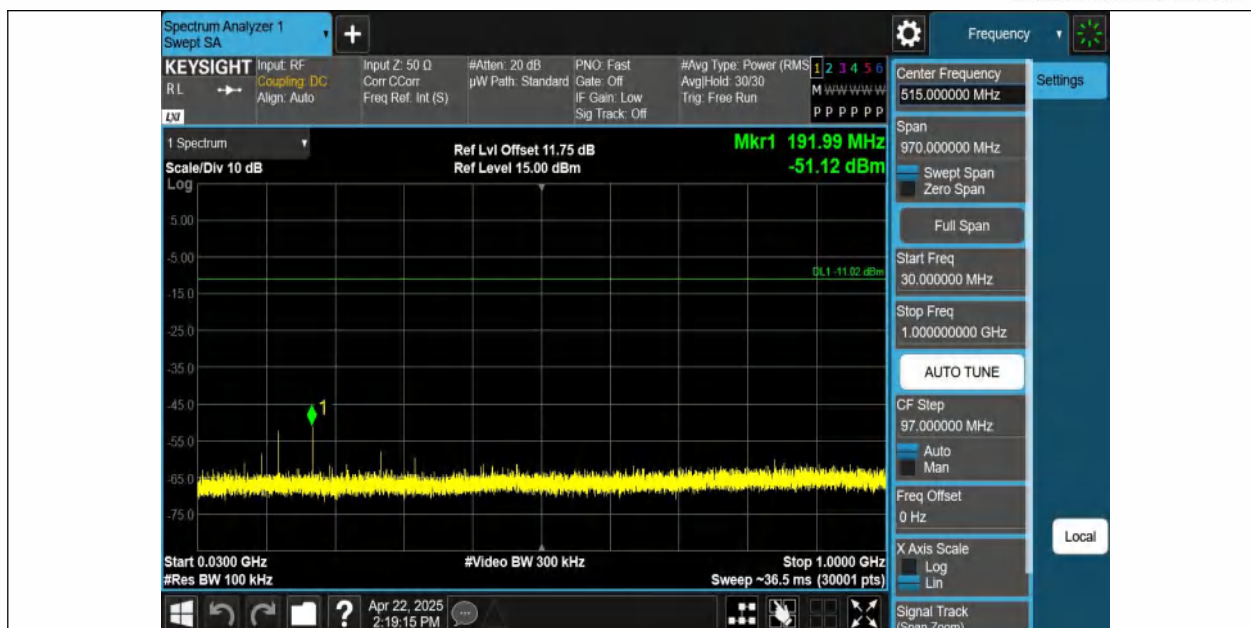
2DH5-Ant1-2402-30~1000-PASS
