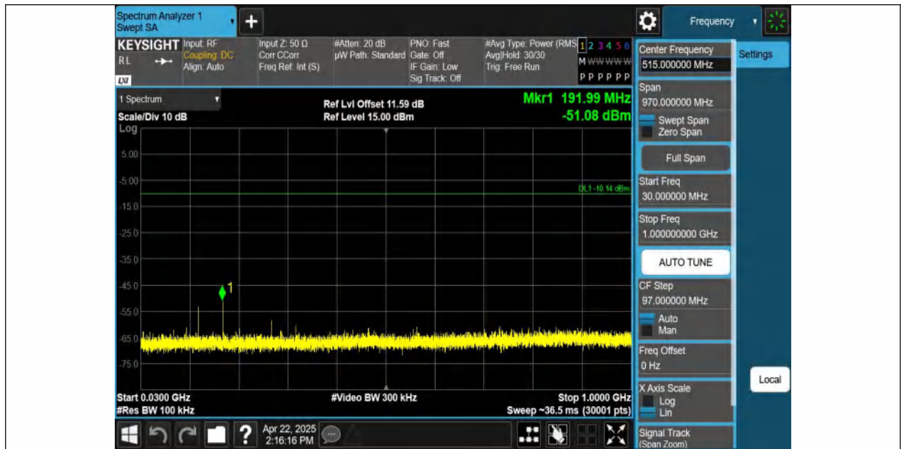
DH5-Ant1-2480-30~1000-PASS
