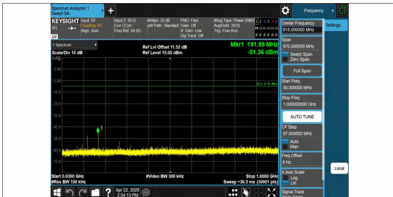
3DH5-Ant1-2441-30~1000-PASS
