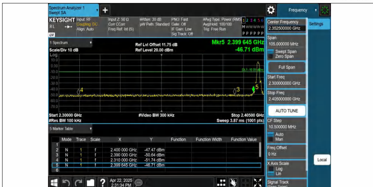
3DH5-Ant1-2402-PASS
