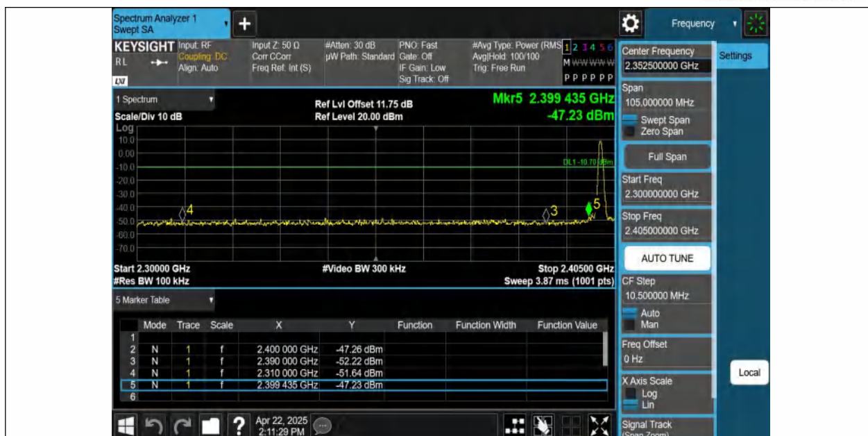
DH5-Ant1-2402-PASS
