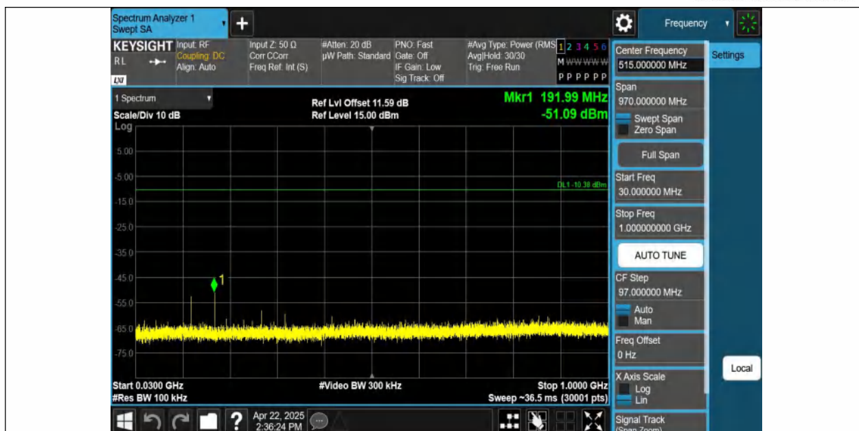
3DH5-Ant1-2480-30~1000-PASS
