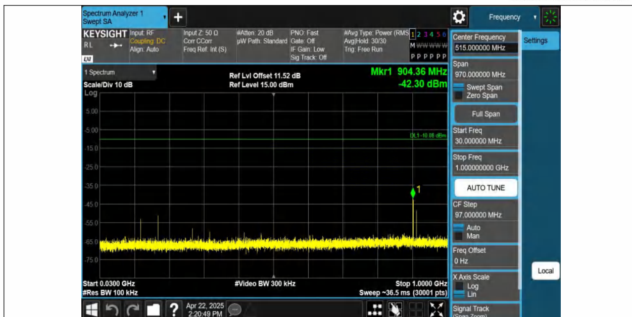
2DH5-Ant1-2441-30~1000-PASS
