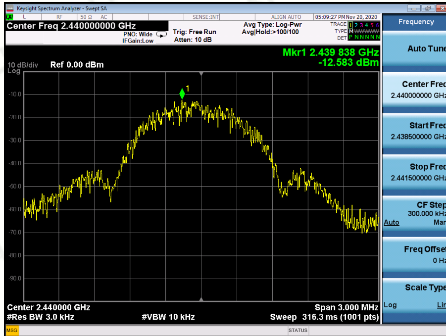
CH: 2440MHz
