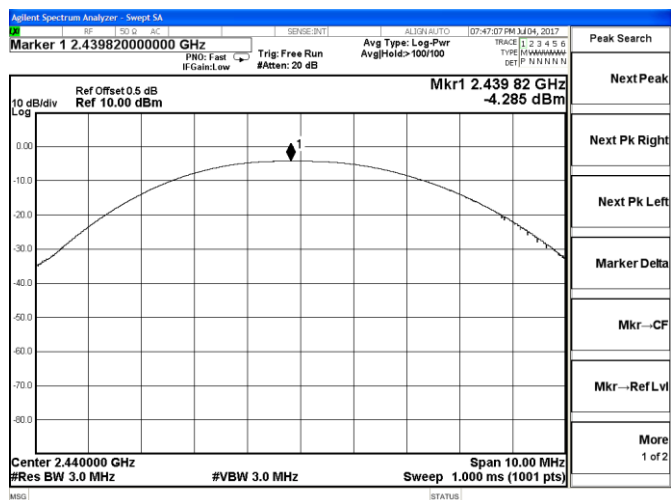
Channel 19 / 2440 MHz
