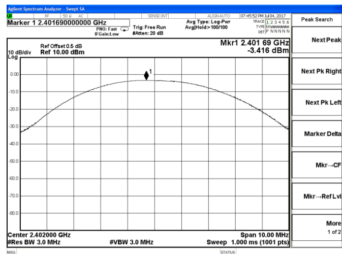
Channel 0 / 2402 MHz
