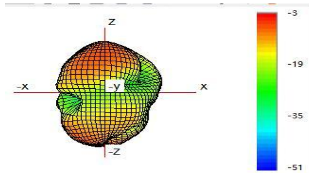
(5) Typical Free Space 3D Radiation Pattern at 2450MHz(unit:dBi)
