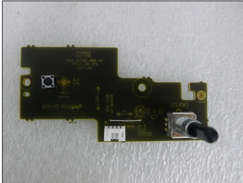
Bottom view of Input SEL PCB
