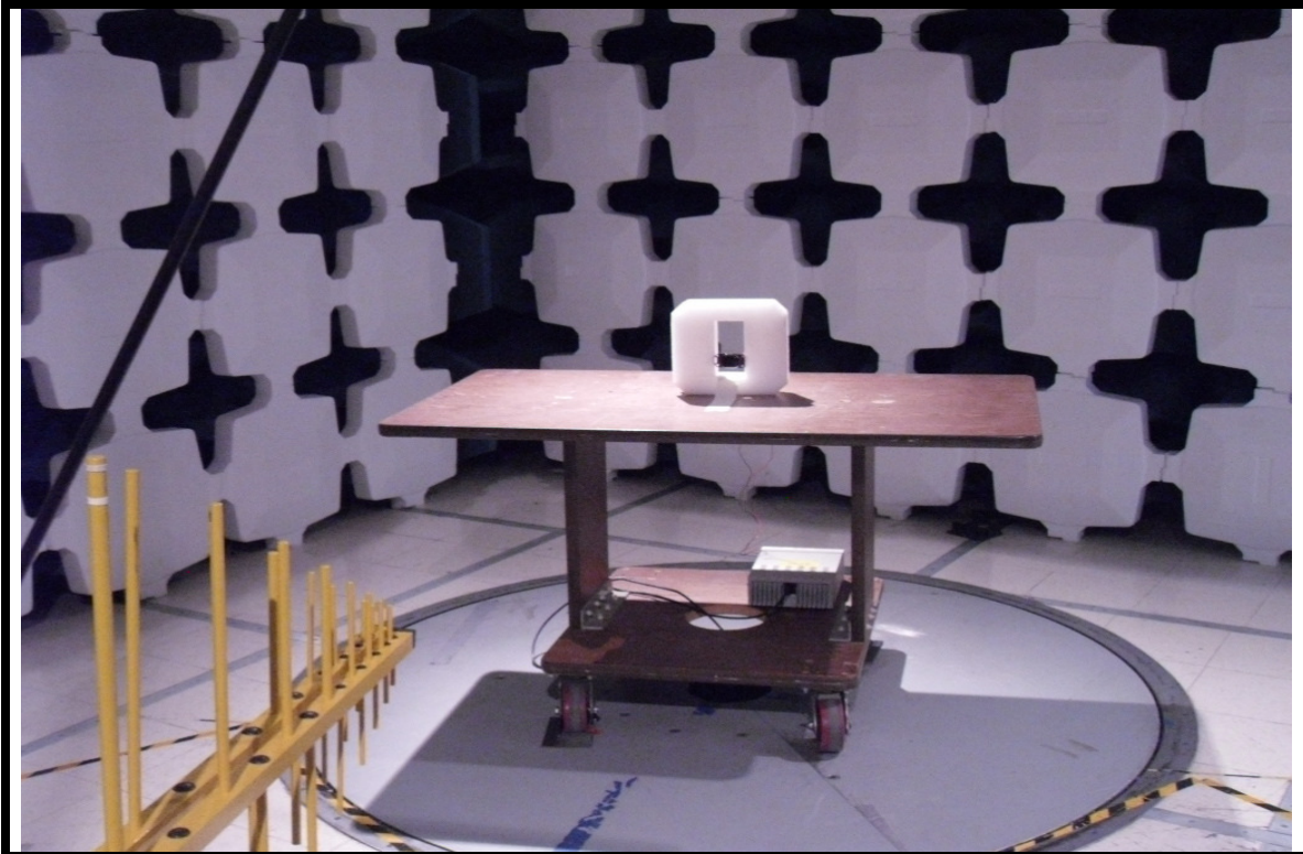
Test Setup Photo # 1
