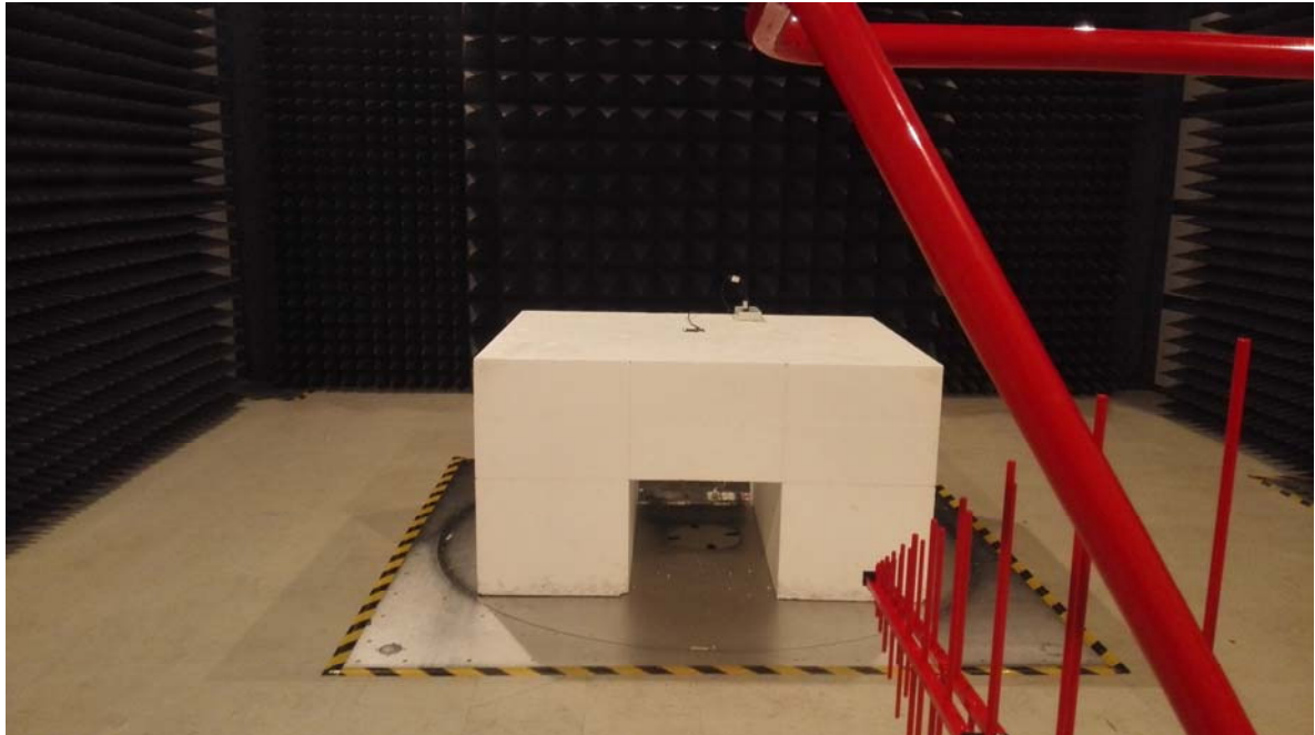
Radiated Spurious Emissions View (Below 1 GHz)
