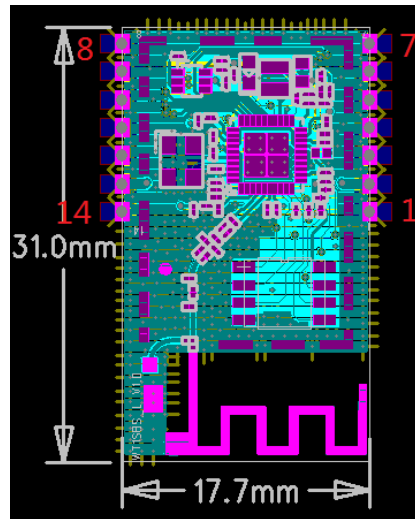
Figure6.WT1SBSLpin-out
