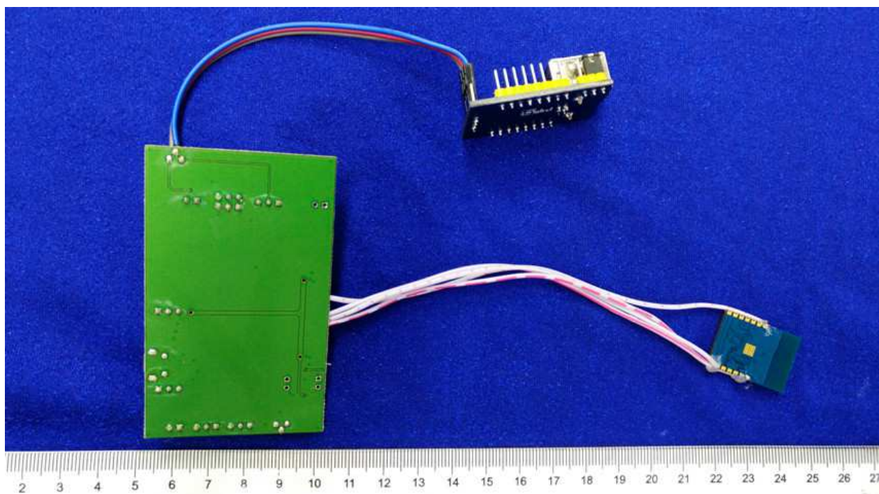
Engineering Board + WIFI module
