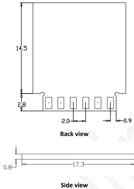
Fig 4 BL3351-P Dimensions
