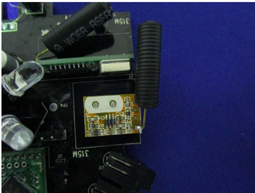
EUT – 315MHz TX Module and Antenna View
