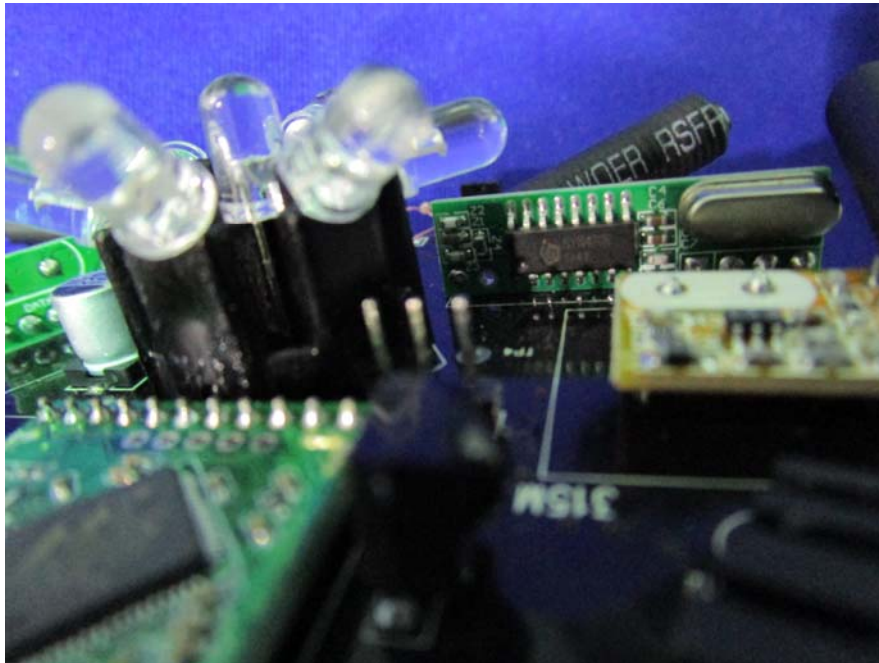
EUT – 315MHz RX Module and Antenna View
