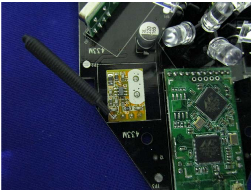
EUT – 433MHz TX Module and Antenna View
