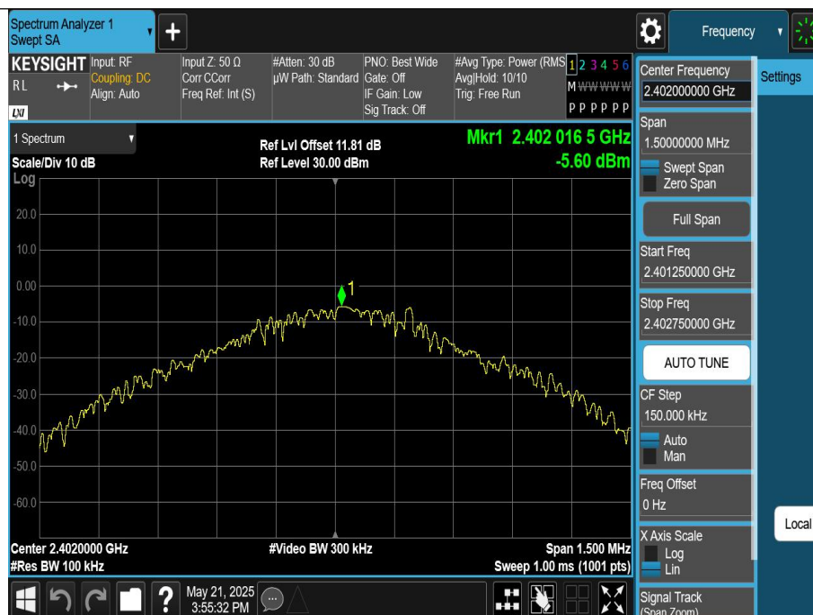
DH5-Ant1-2402-0~Reference-PASS
