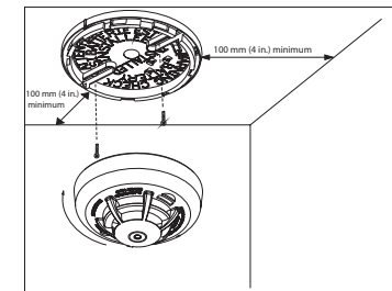
Fig 9. Mounting the detector
