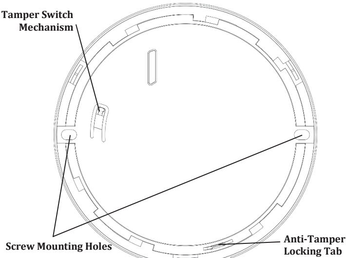
Figure 3 - Mounting Base
