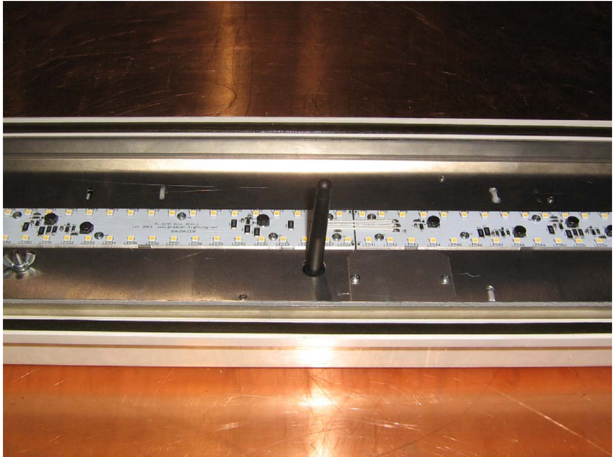
LED Assembly with heatsink and electronics installed showing Antenna and factory access port
