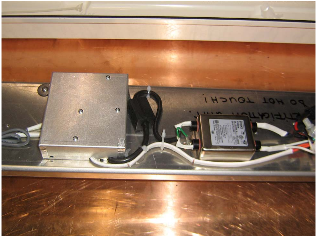
RF Subunit mounted inside of LED Light assembly attached to heatsink
