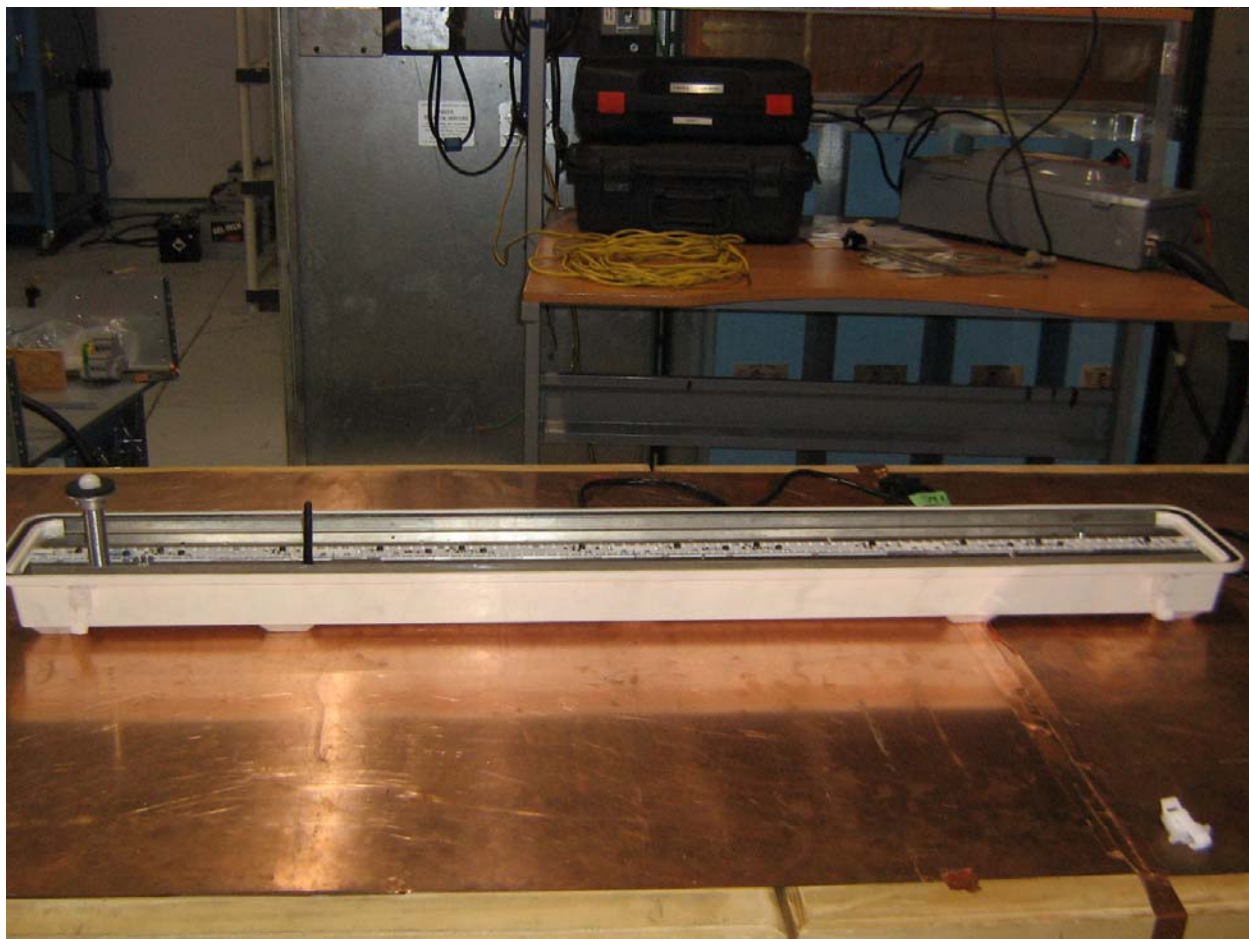
LED Assembly with heatsink and electronics installed showing Antenna and Motion Sensor
