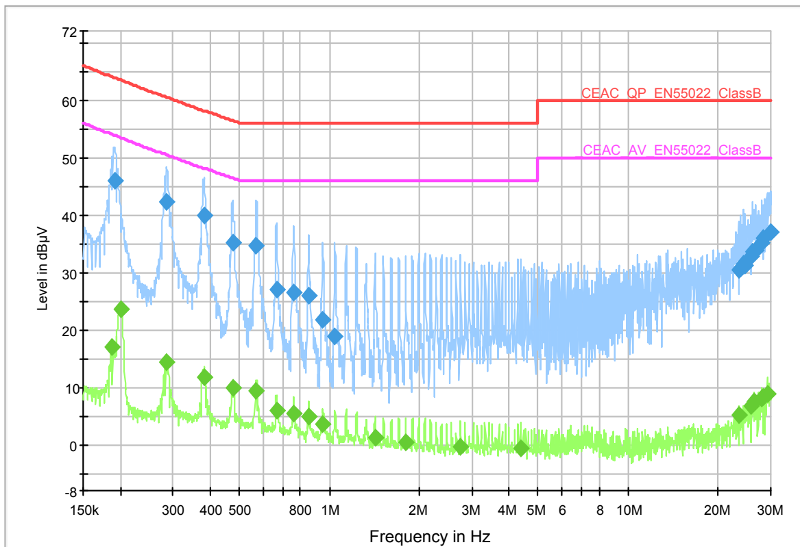
Figure 4: AC Conducted Emissions - Line 2 240VAC/60Hz (Idle Mode)
