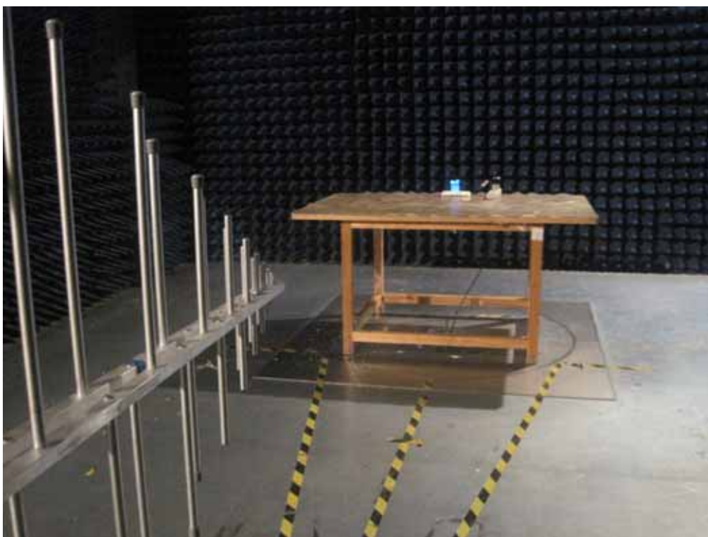
Test frequency from 1GHz~25GHz
