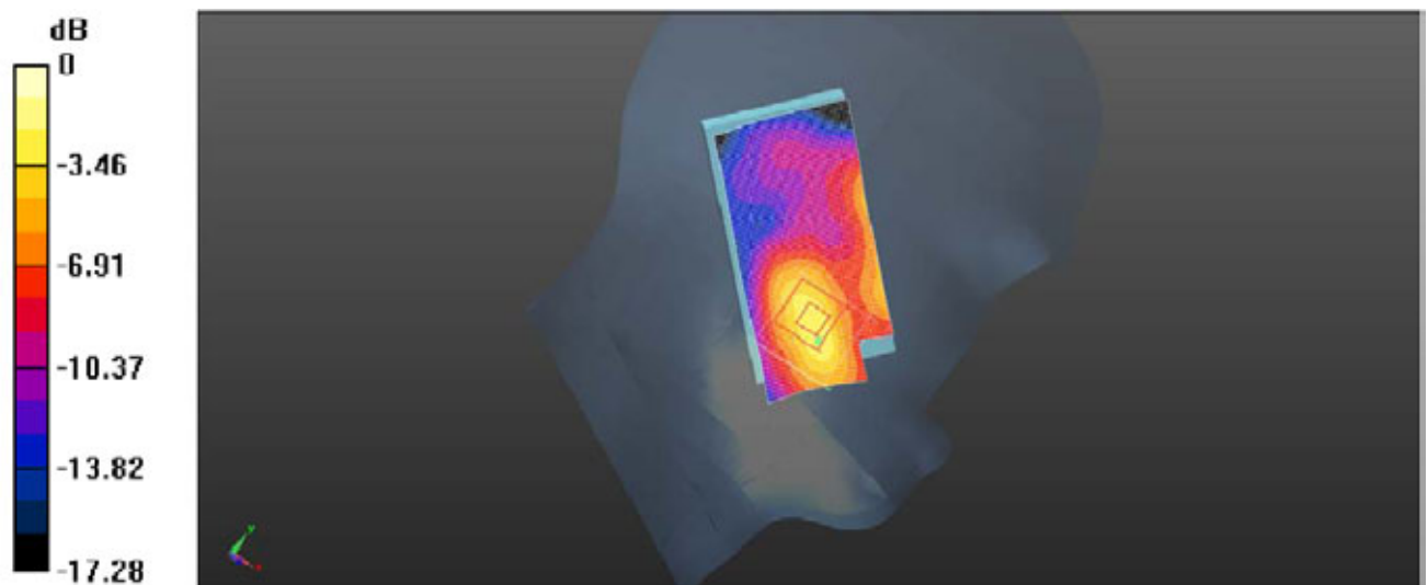
Plot 3: Left Head Touch (PCS1900 Middle Channel)
