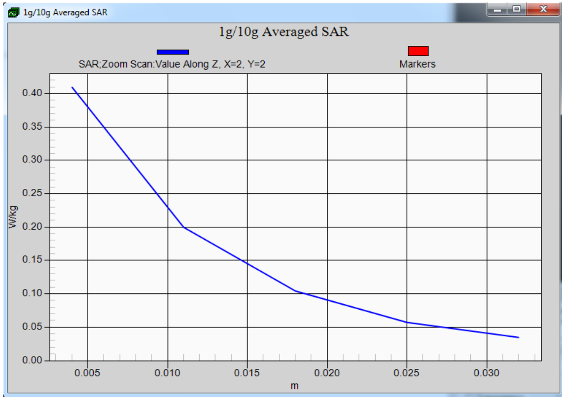
Z-Scan at power reference point- Left Head Touch (GSM850 Middle Channel)
