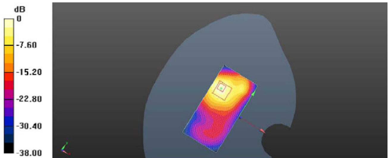
Plot 6: Rear Side (WLAN2450-Middle Channel-Channel 6-2437MHz)
