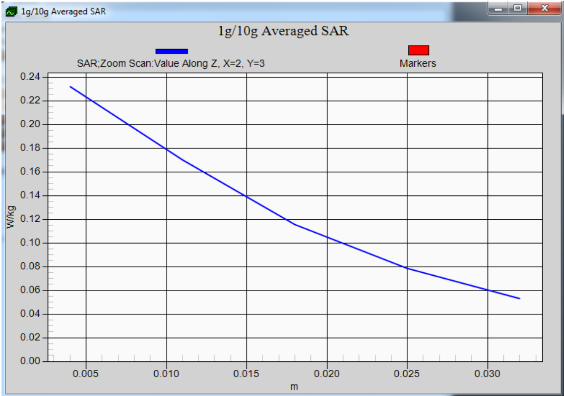
Z-Scan at power reference point- Rear Side (WLAN2450-Middle Channel-Channel 6-2437MHz)
