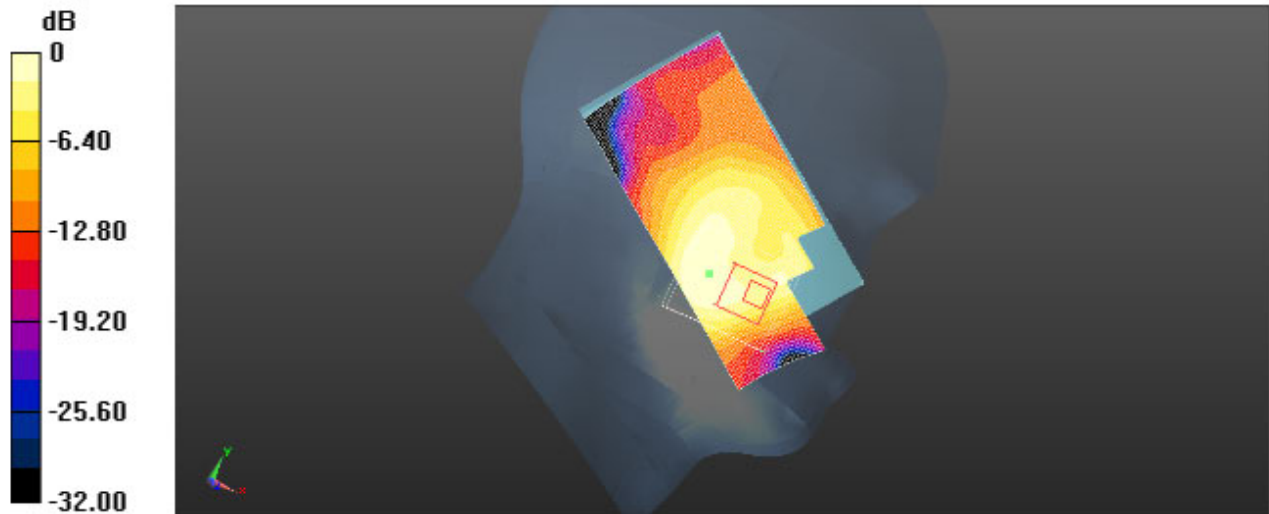
Plot 5: Left Head Touch (WLAN2450-Middle Channel-Channel 6-2437MHz)
