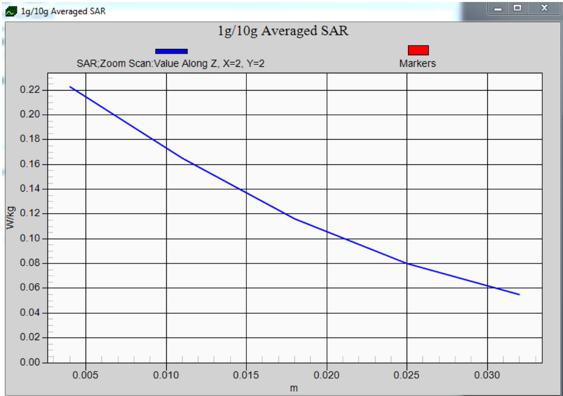
Z-Scan at power reference point- Left Head Touch (WLAN2450-Middle Channel-Channel 6-2437MHz)
