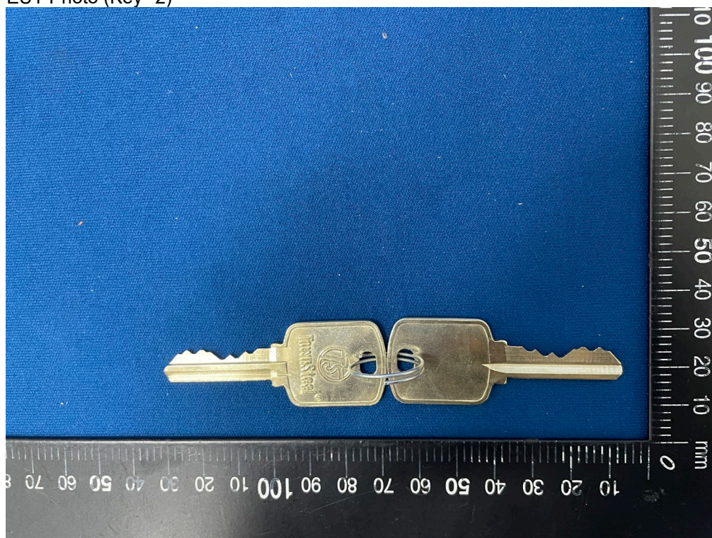
(7) EUT Photo (Key* 2)
