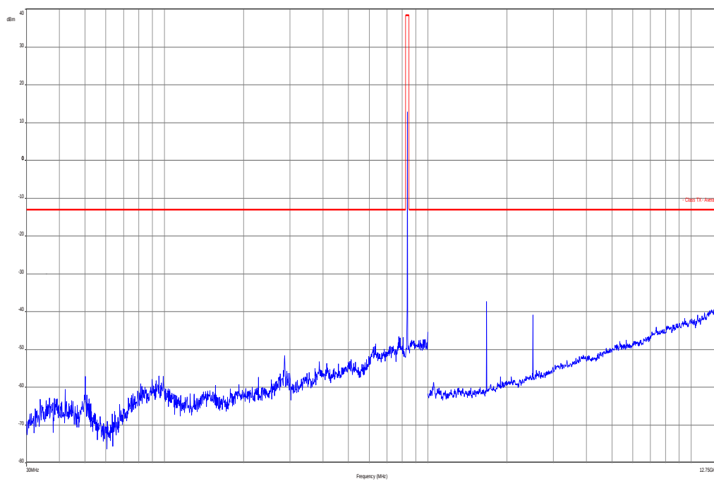
Plot 2: Channel 189 (GMSK modulation, 30 MHz – 12.75 GHz)
