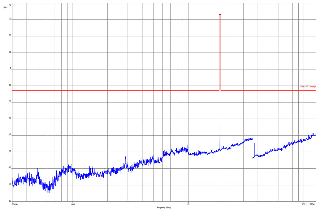
Plot 5: Channel 661 (8-PSK modulation, 30 MHz – 12.75 GHz)
