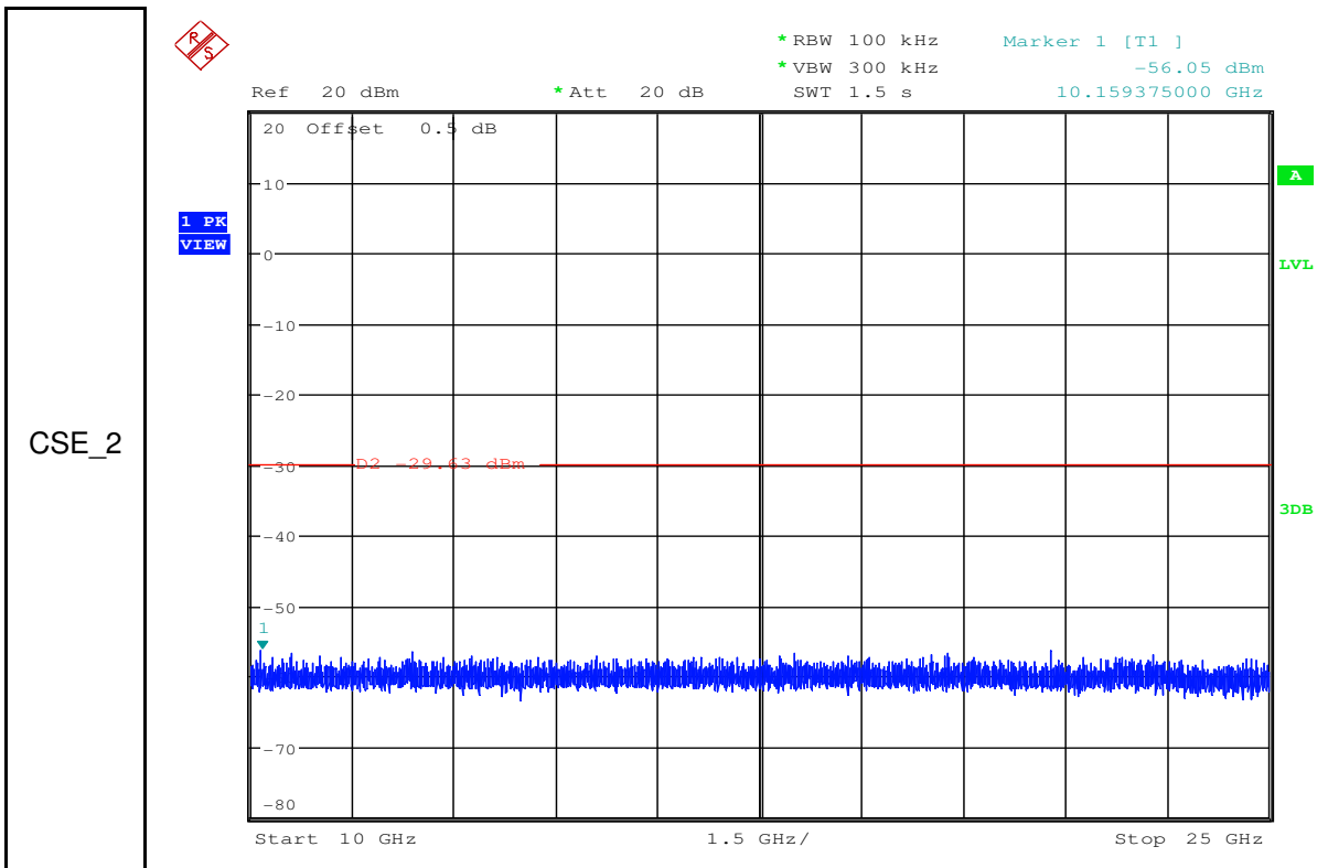
RF Conducted Spurious Emissions_11N20SISO_2412_Ant1
