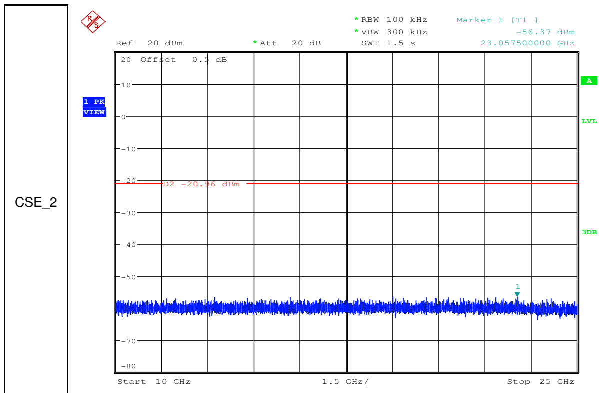
RF Conducted Spurious Emissions_11N20SISO_2462_Ant1
