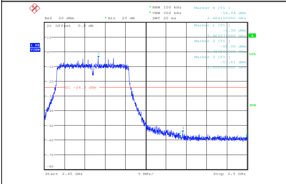
Band-edge for RF Conducted Emissions_11N20SISO_2462_Ant1
