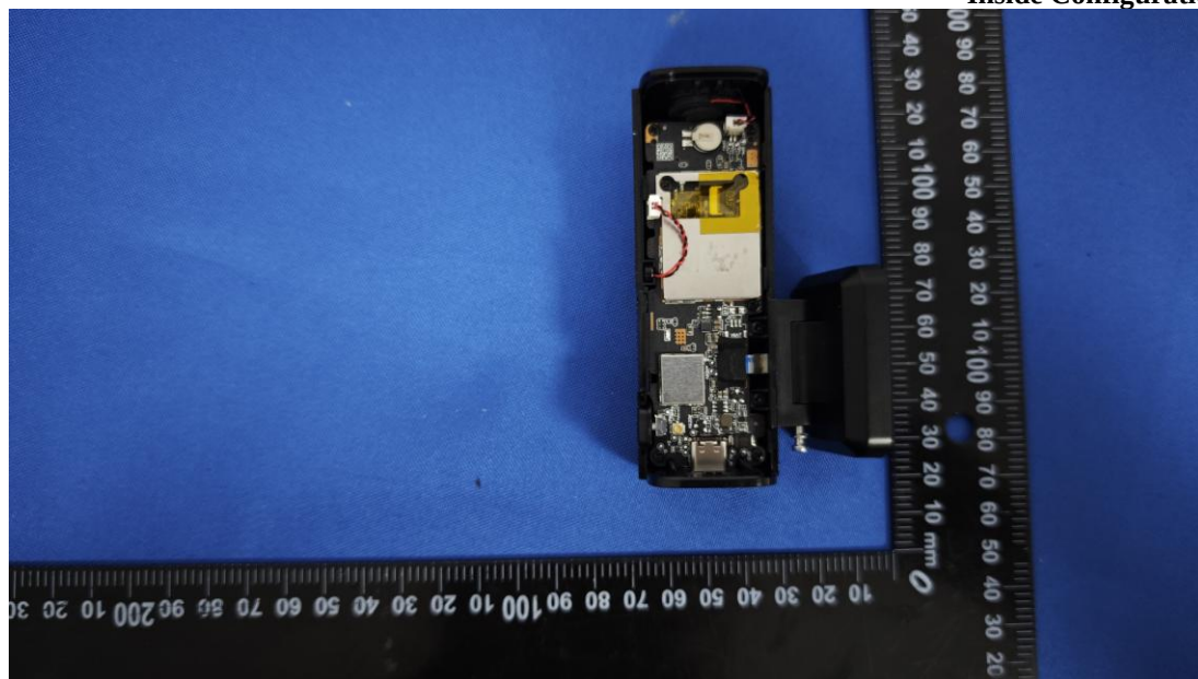
Figure 12 Inside Configuration of the EUT
