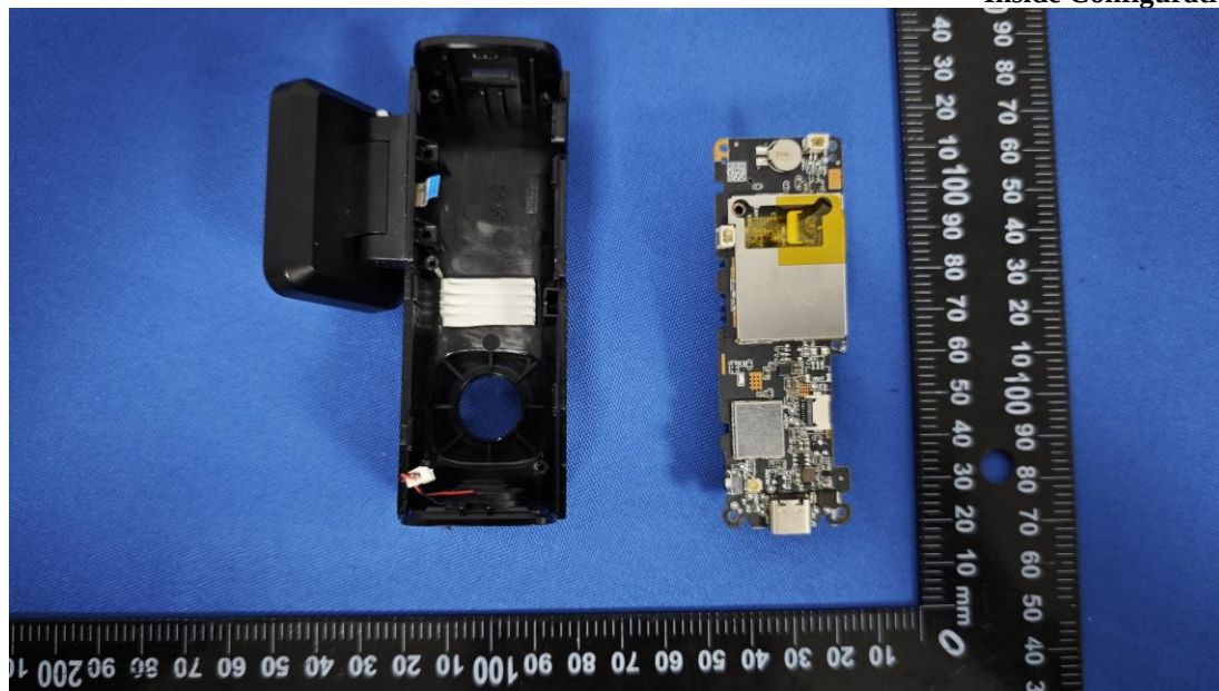
Figure 11 Inside Configuration of the EUT
