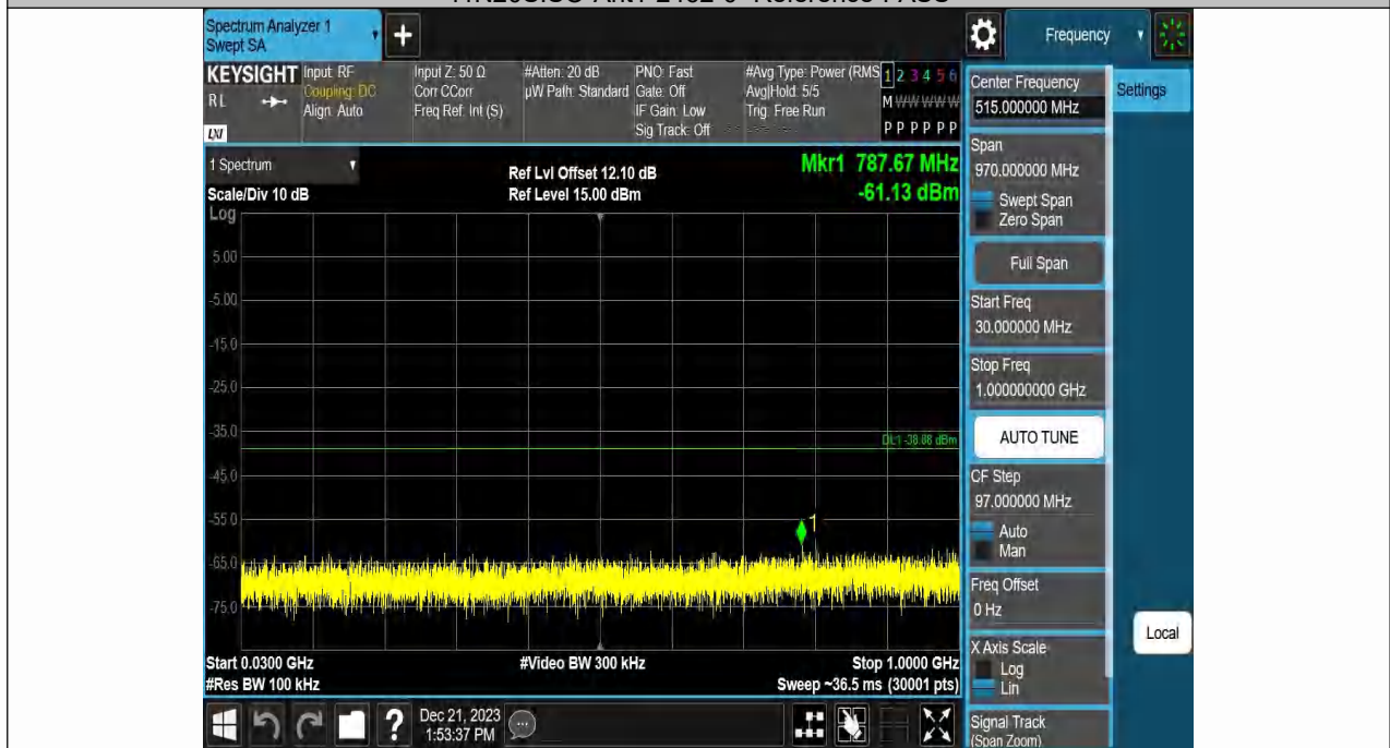
11N20SISO-Ant1-2462-30~1000-PASS
