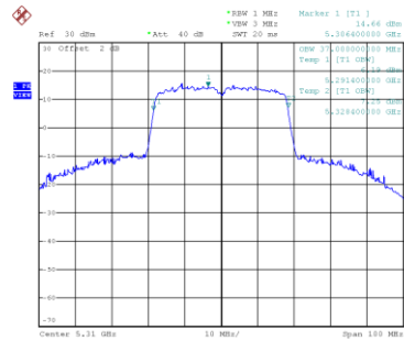
99 % Emission Bandwidth
