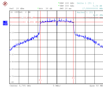
6 dB Bandwidth
