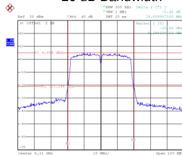
26 dB Bandwidth
