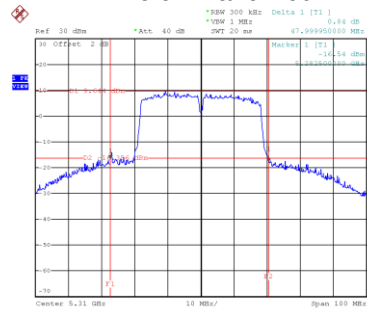
26 dB Bandwidth
