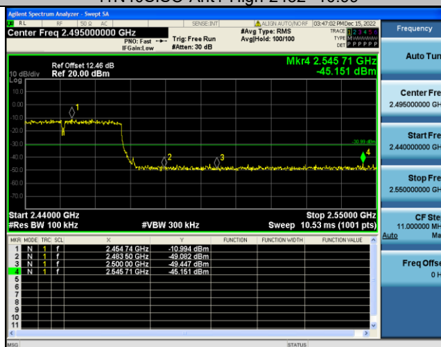
11N40SISO-Ant1-High-2452--10.99
