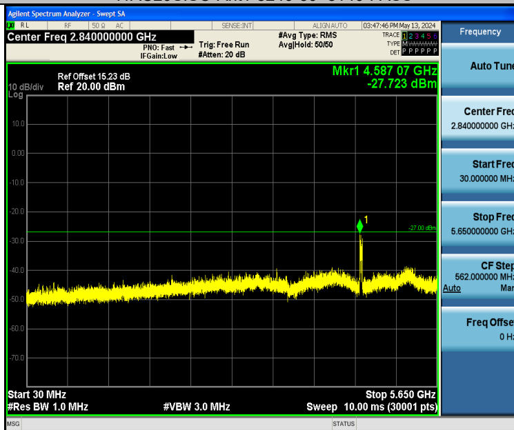
11N40SISO-Ant1-5755-30~5650-PASS
