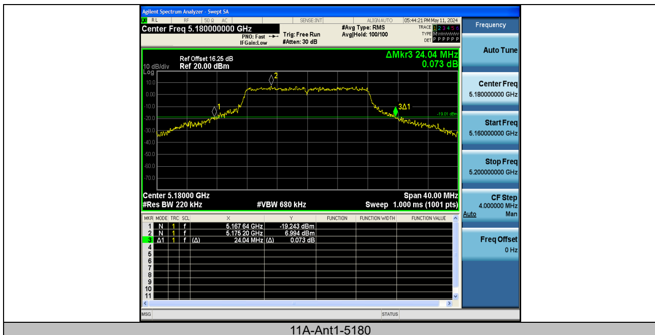
11A-Ant1-5180
