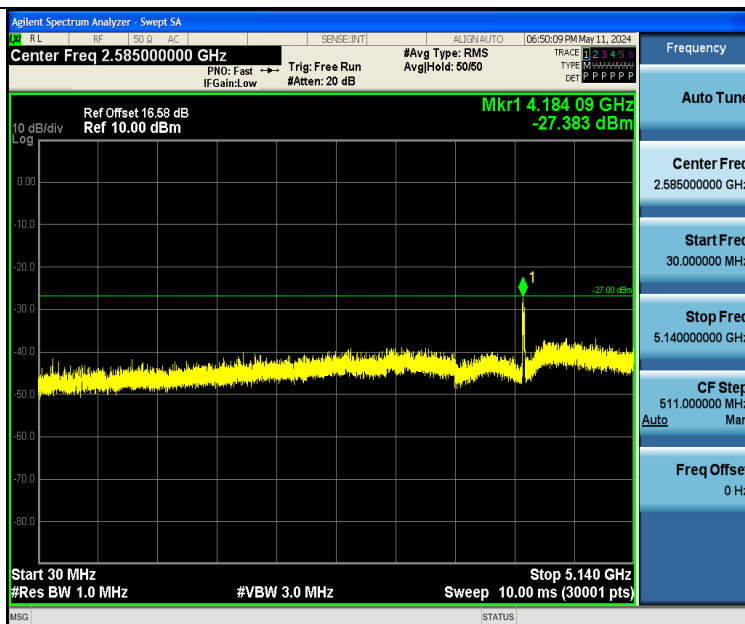
11AC20SISO-Ant1-5240-30~5140-PASS
