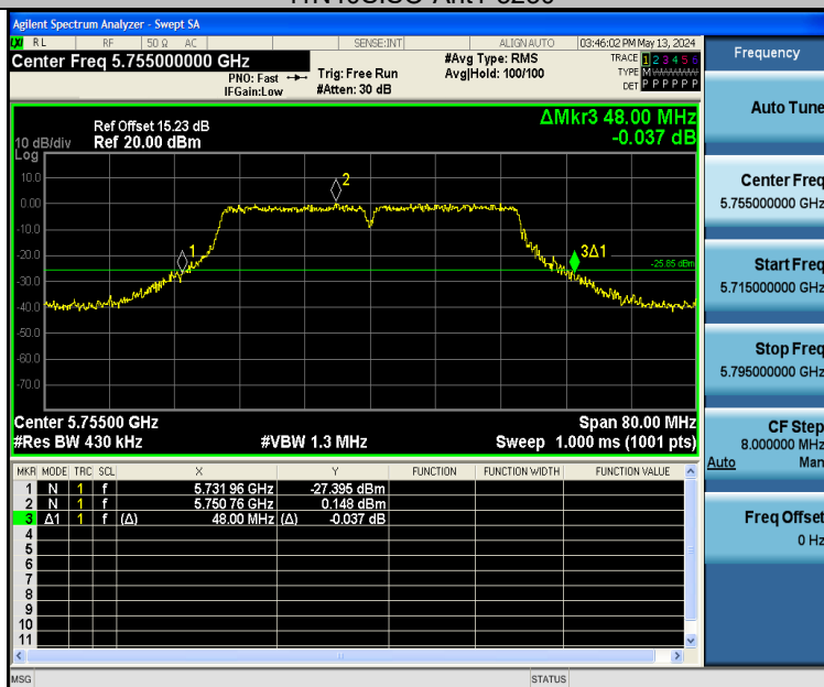
11N40SISO-Ant1-5755
