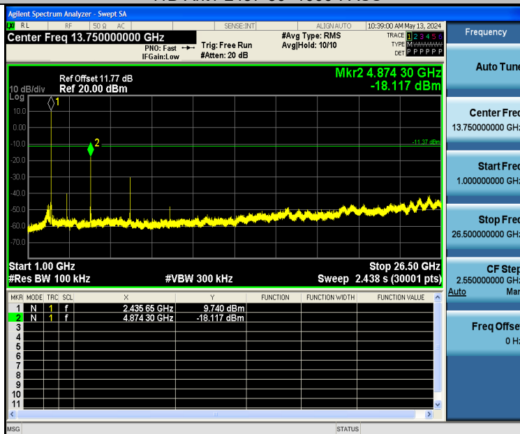
11B-Ant1-2437-1000~26500-PASS
