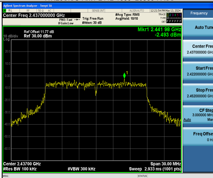
11N20SISO-Ant1-2437-0~Reference-PASS
