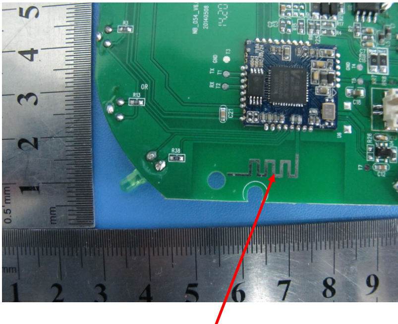
PCB BT Antenna
