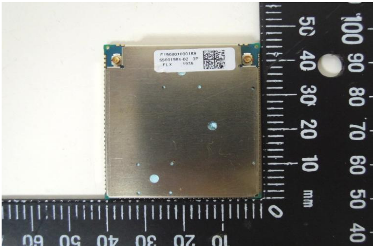
Front view ConnectCore 8X
