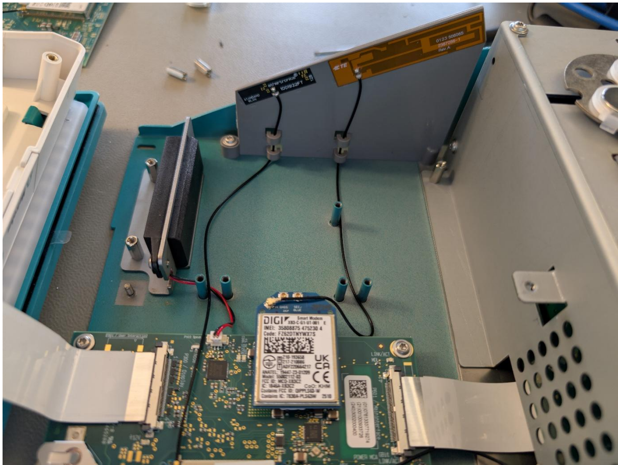
Antenna assembly left (LTE & WLAN/BT secondary antenna)
