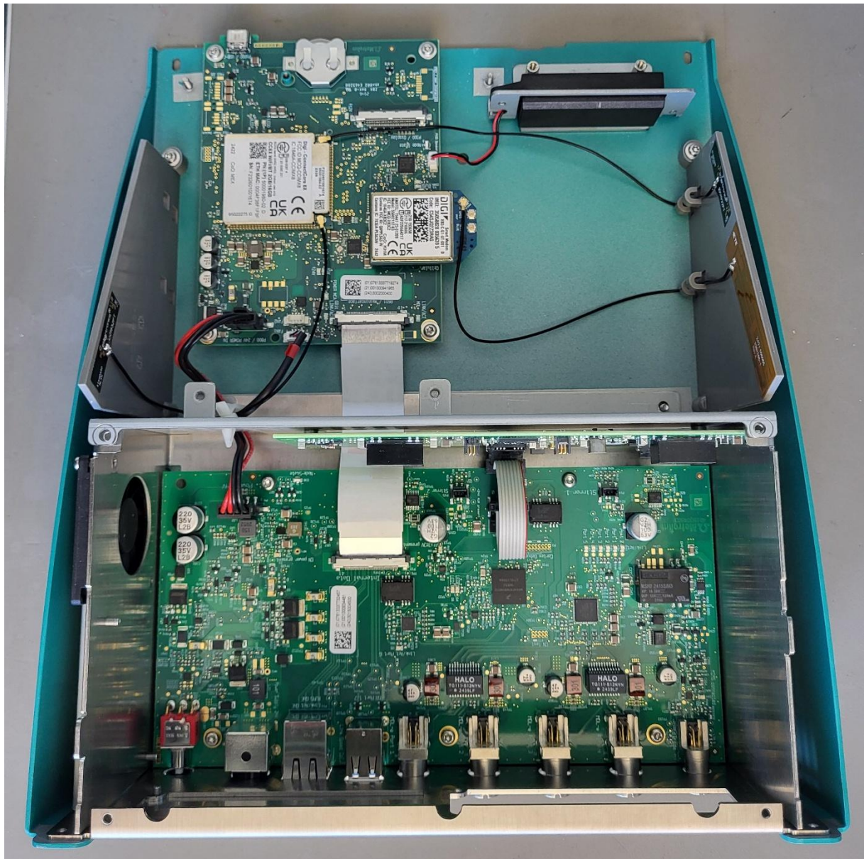
Electronic Box (without shield)
