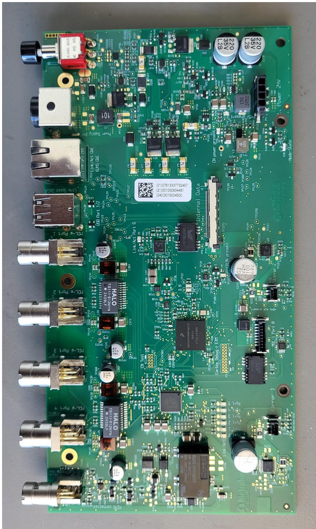
PCBA Main Interface CN (top side)
