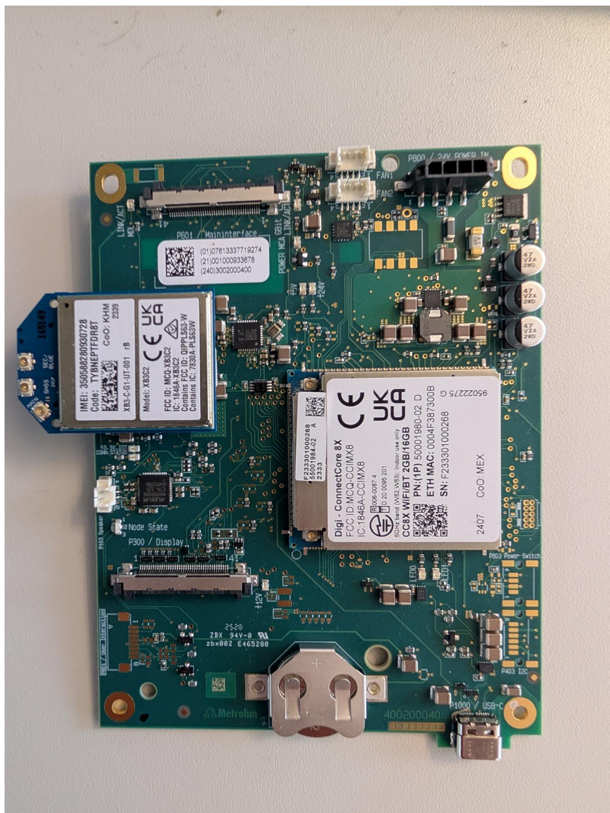
PCBA Mainboard MN (top side)
