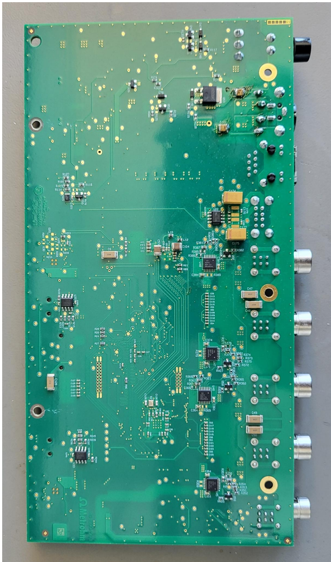
PCBA Main Interface CN (bottom side)
