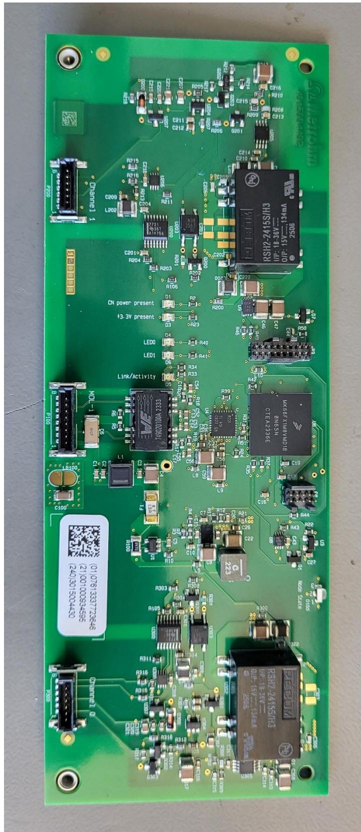
PCBA Meas Interface CN (top side)
