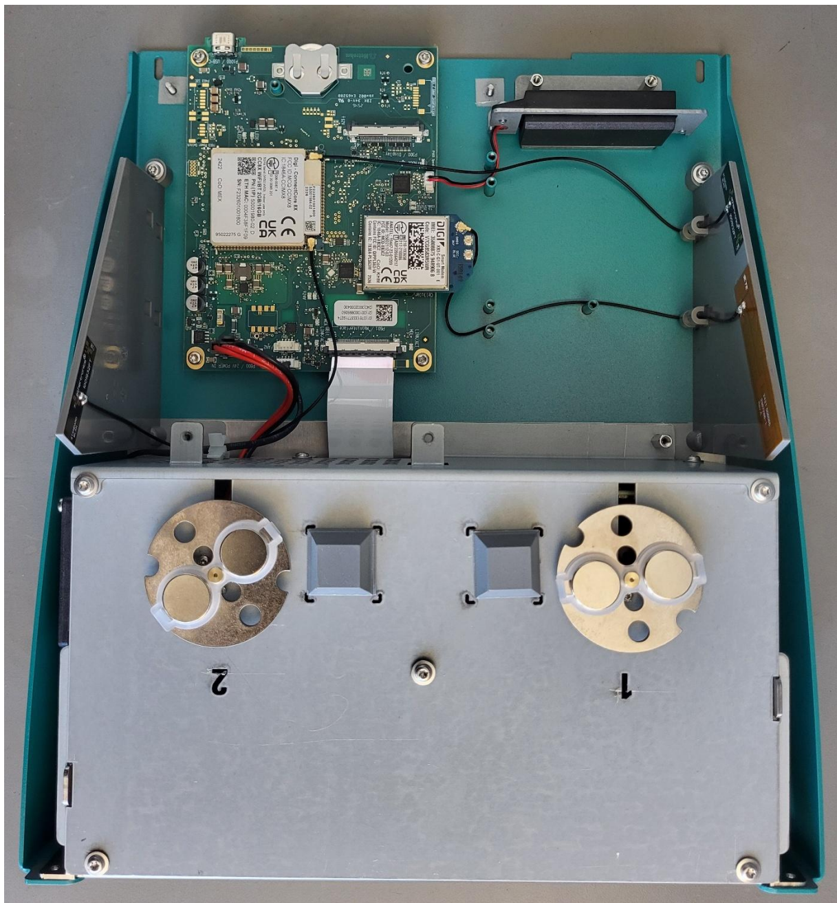
Mainboard (without shield)
