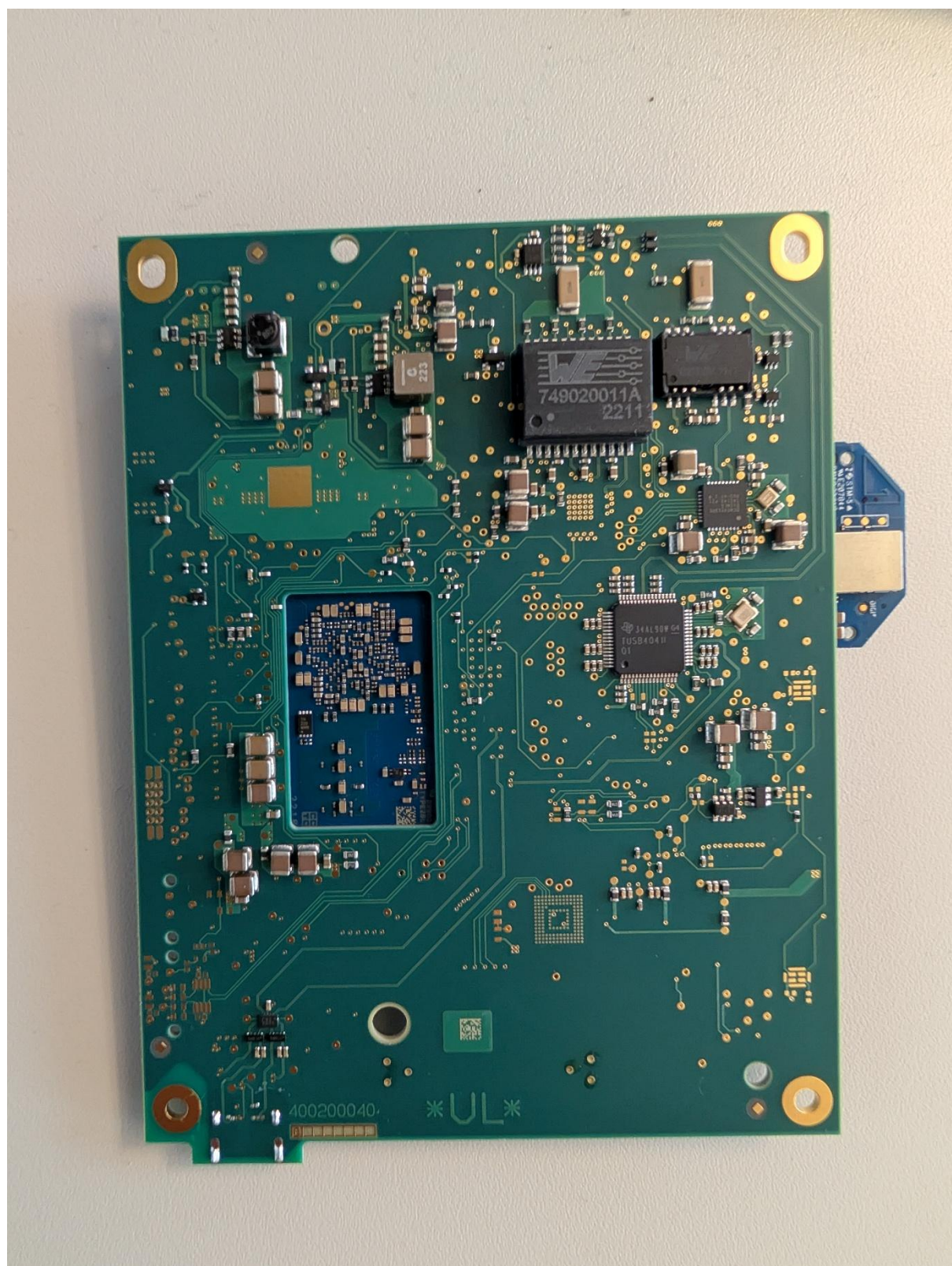
PCBA Mainboard MN (bottom side)
