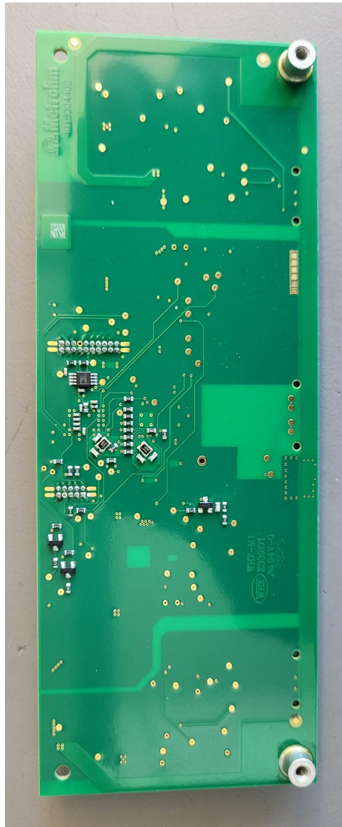
PCBA Meas Interface CN (bottom side)
