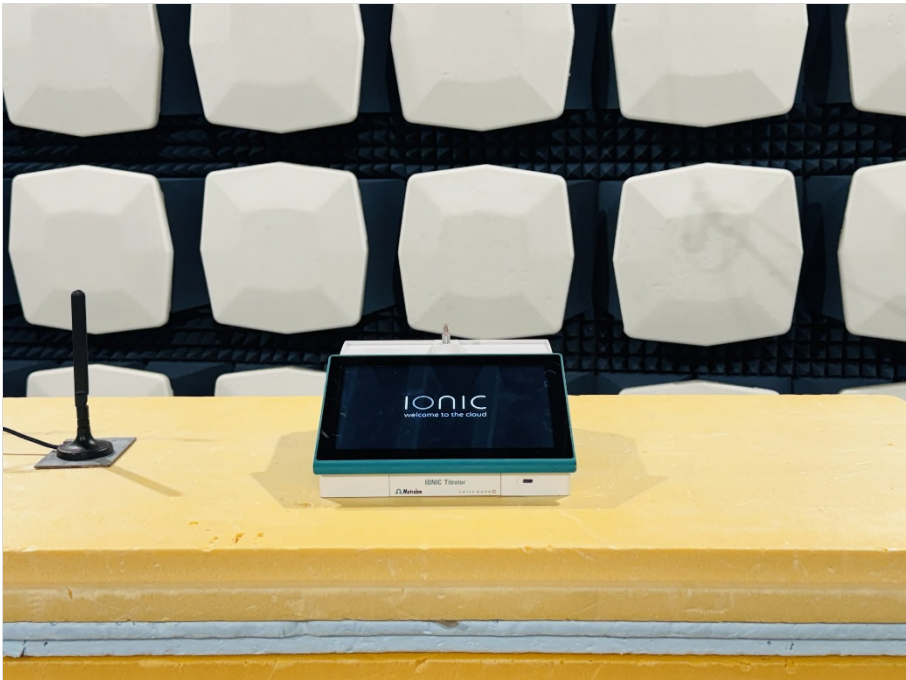
Photograph 2: EUT test setup in the fully anechoic chamber, close up view_EUT elevation 0°
