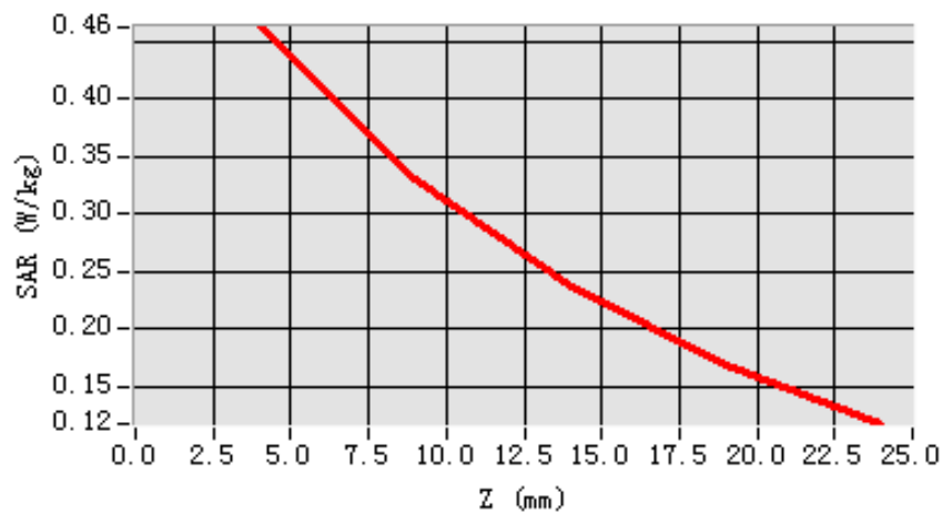
SAR, Z Axis Scan (X = -29, Y = -11)
