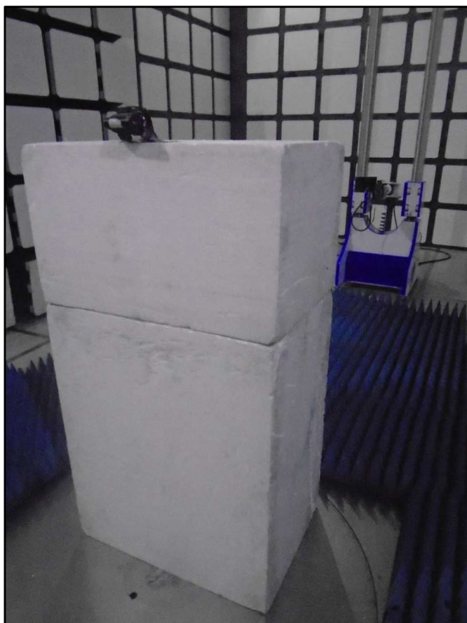
Figure 27 - 1 GHz to 10 GHz - Z Orientation
