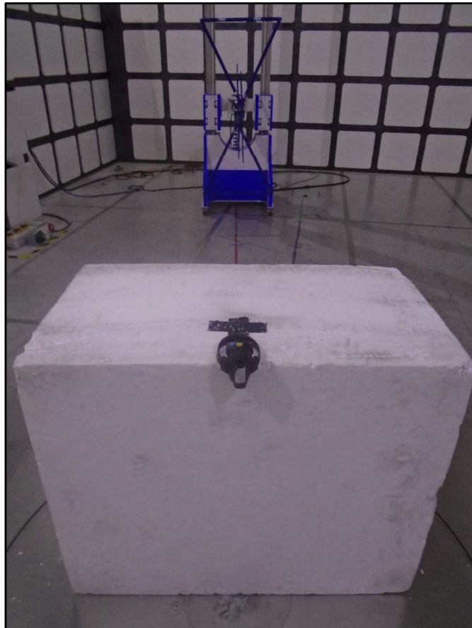
Figure 23 - 30 MHz to 1 GHz - Y Orientation
