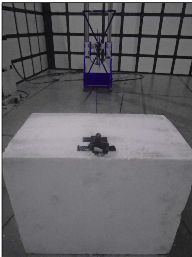
Figure 24 - 30 MHz to 1 GHz - Z Orientation
