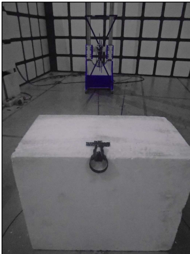
Figure 22 - 30 MHz to 1 GHz - X Orientation
