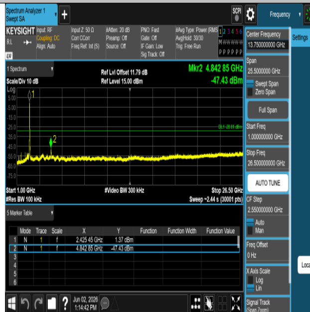
11AX40SISO-Ant1-2422-1000~26500-PASS
