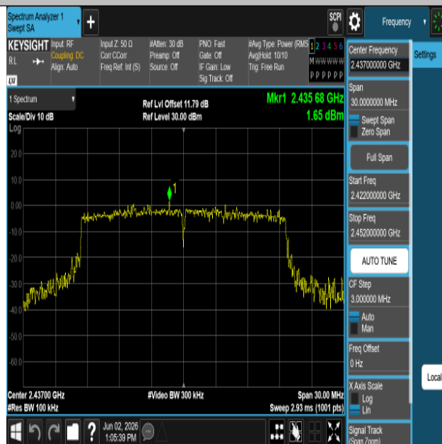
11AX20SISO-Ant1-2437-0~Reference-PASS
