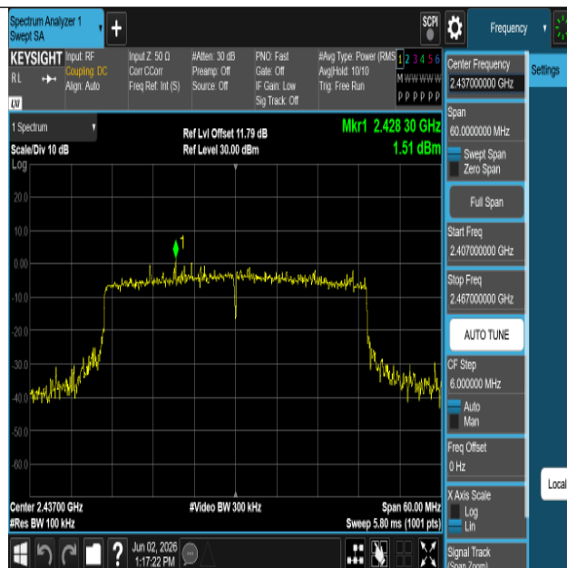
11AX40SISO-Ant1-2437-0~Reference-PASS
