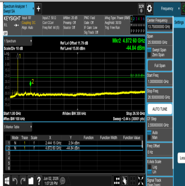
11AX20SISO-Ant1-2437-1000~26500-PASS
