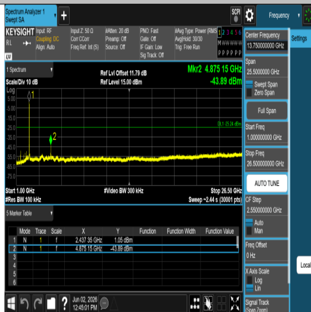
11N20SISO-Ant1-2437-1000~26500-PASS
