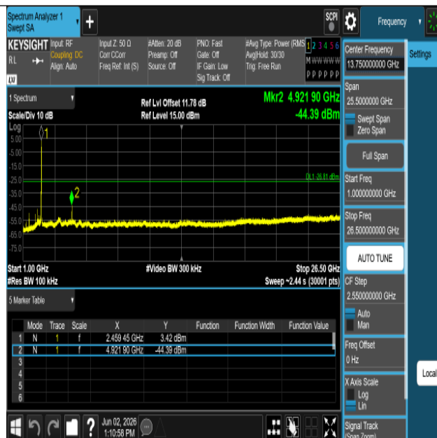
11AX20SISO-Ant1-2462-1000~26500-PASS
