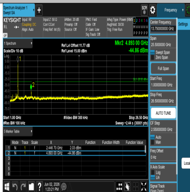
11AX40SISO-Ant1-2452-1000~26500-PASS
