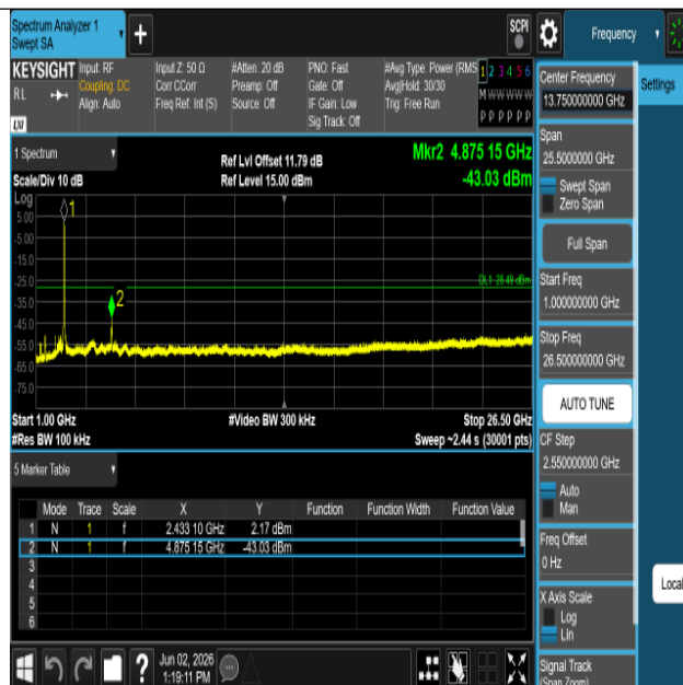
11AX40SISO-Ant1-2437-1000~26500-PASS
