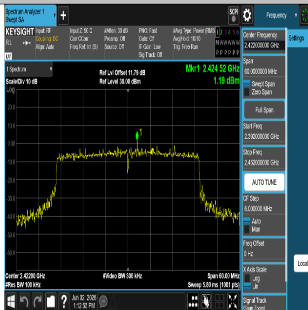
11AX40SISO-Ant1-2422-0~Reference-PASS
