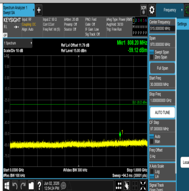
11N40SISO-Ant1-2437-30~1000-PASS
