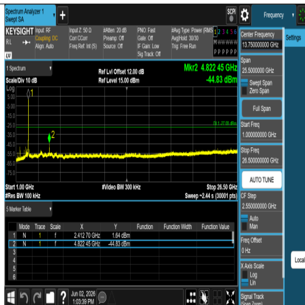
11AX20SISO-Ant1-2412-1000~26500-PASS
