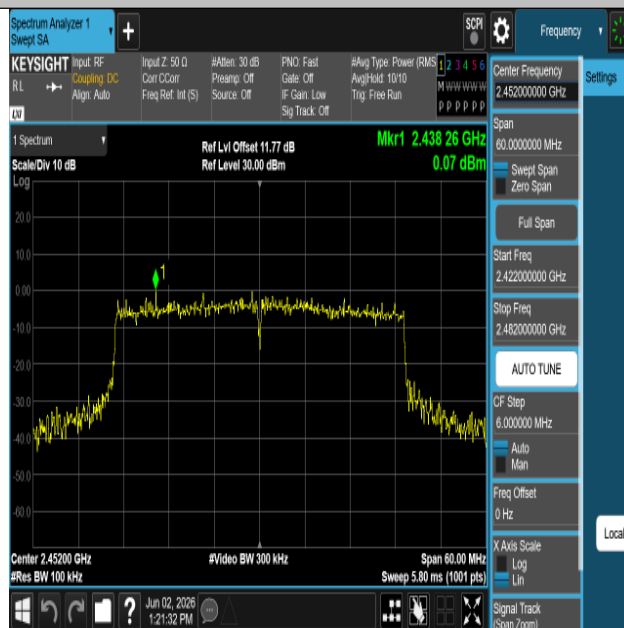
11AX40SISO-Ant1-2452-0~Reference-PASS
