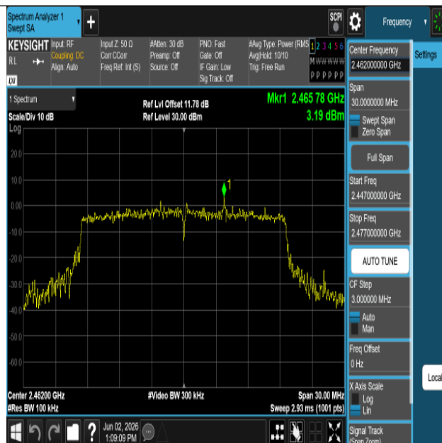
11AX20SISO-Ant1-2462-0~Reference-PASS
