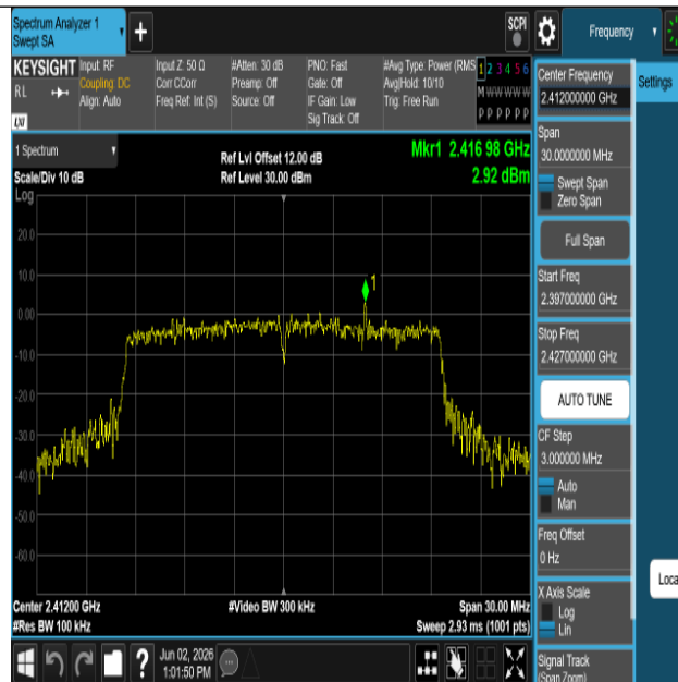
11AX20SISO-Ant1-2412-0~Reference-PASS
