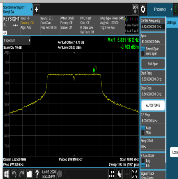
11A-Ant1-5825-PASS
