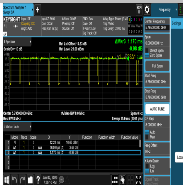
NTNV-11AC40SISO-Ant1-5795
