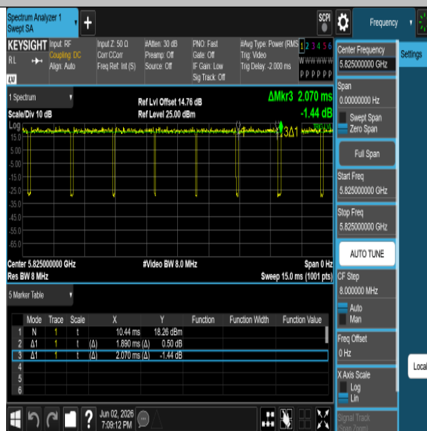
NTNV-11AC20SISO-Ant1-5825
