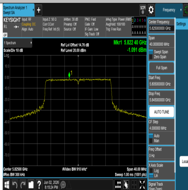
11AX20SISO-Ant1-5825-PASS
