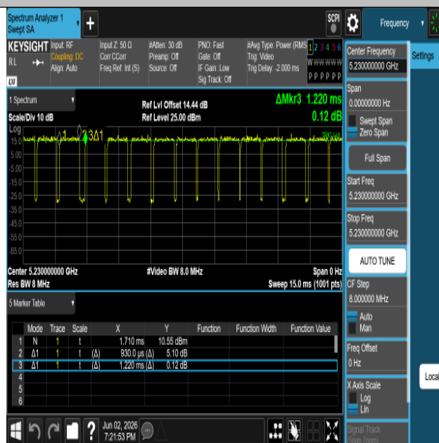
NTNV-11AC40SISO-Ant1-5230
