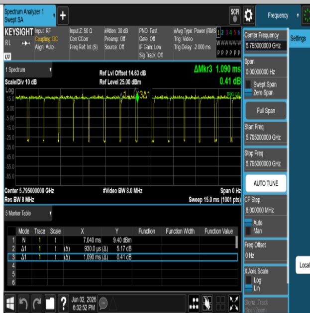
NTNV-11N40SISO-Ant1-5795
