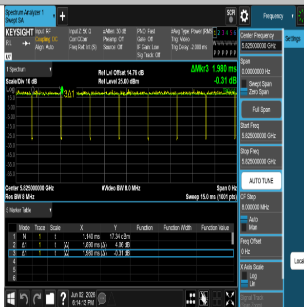
NTNV-11N20SISO-Ant1-5825
