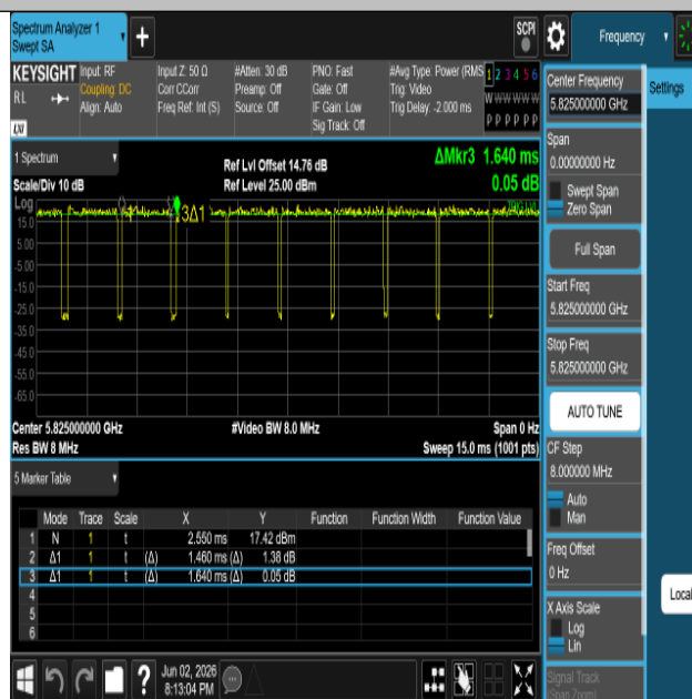
NTNV-11AX20SISO-Ant1-5825
