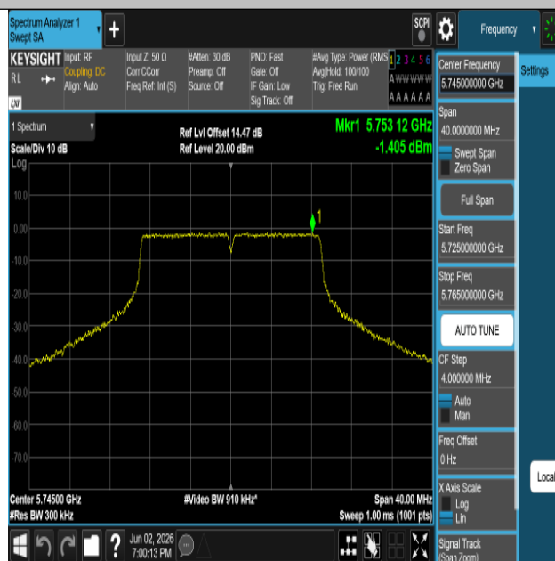
11AC20SISO-Ant1-5745-PASS
