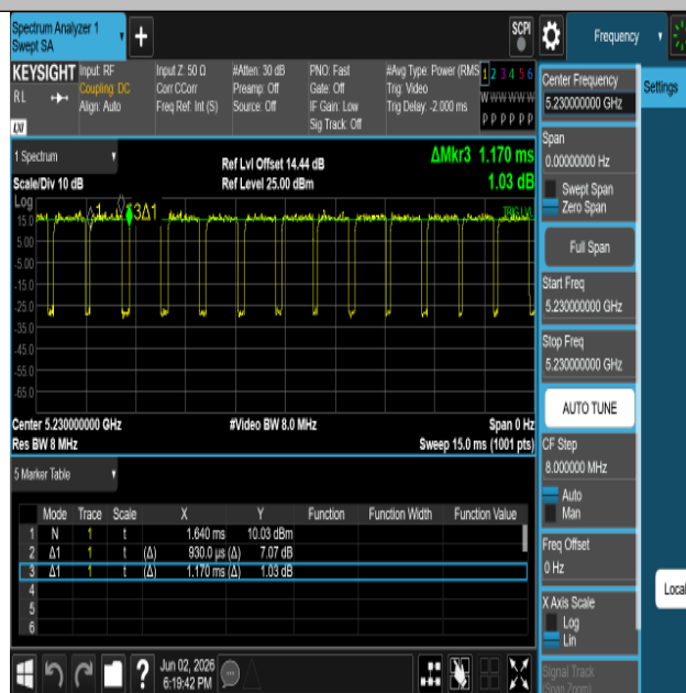
NTNV-11N40SISO-Ant1-5230
