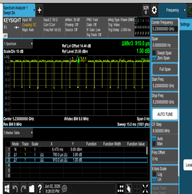
NTNV-11AX40SISO-Ant1-5230
