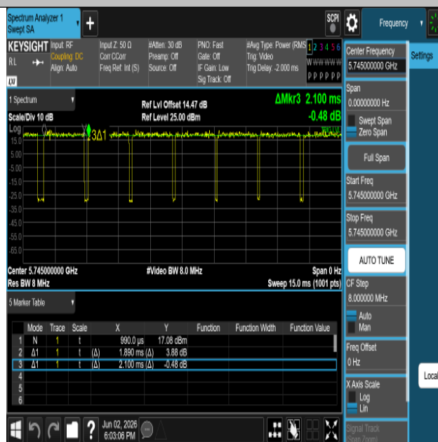
NTVN-11N20SISO-Ant1-5745
