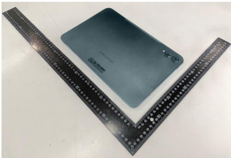
EUT PHOTO 8-External view for mode TLA016
