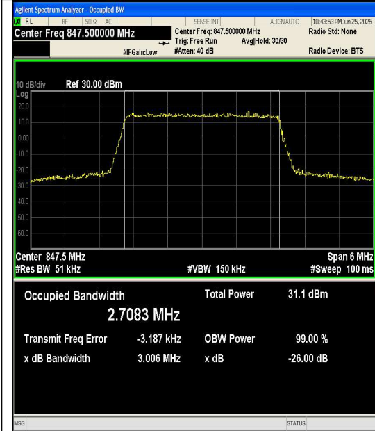
Band5-3MHz-QPSK-20635-15RB#0-PASS
