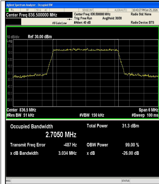
Band5-3MHz-QPSK-20525-15RB#0-PASS
