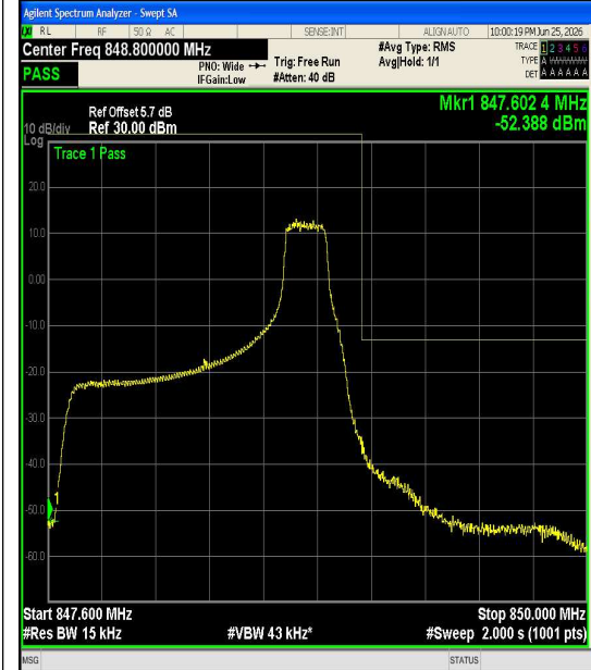
Band5-1.4MHz-QPSK-20643-1RB#5-PASS
