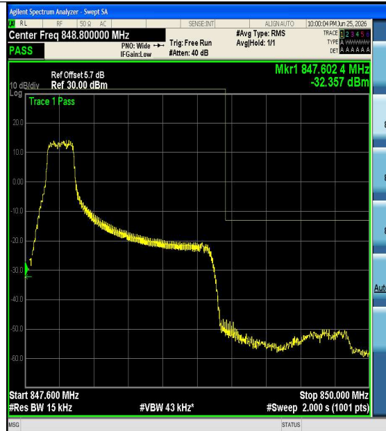
Band5-1.4MHz-16QAM-20643-1RB#0-PASS
