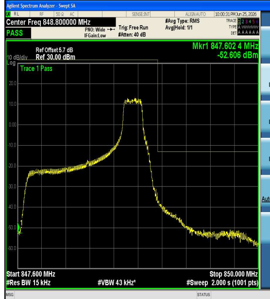
Band5-1.4MHz-16QAM-20643-1RB#5-PASS
