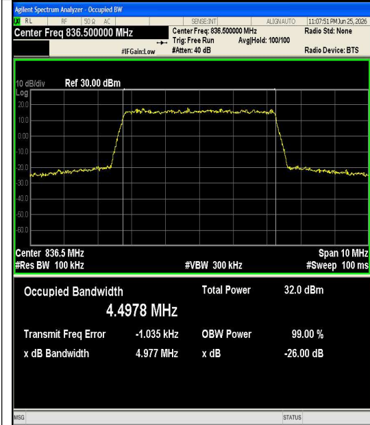
Band5-5MHz-QPSK-20525-25RB#0-PASS
