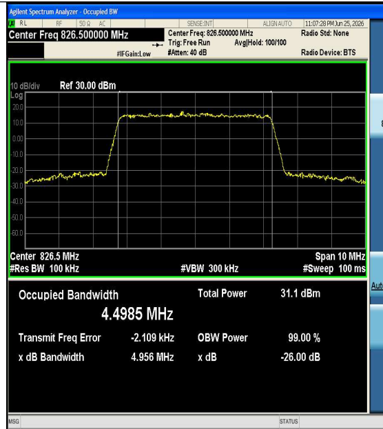
Band5-5MHz-16QAM-20425-25RB#0-PASS
