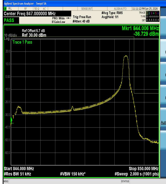
Band5-5MHz-16QAM-20625-1RB#24-PASS
