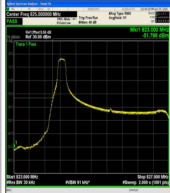
Band5-3MHz-QPSK-20415-1RB#0-PASS
