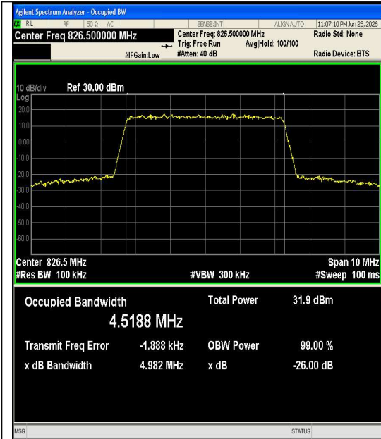
Band5-5MHz-QPSK-20425-25RB#0-PASS
