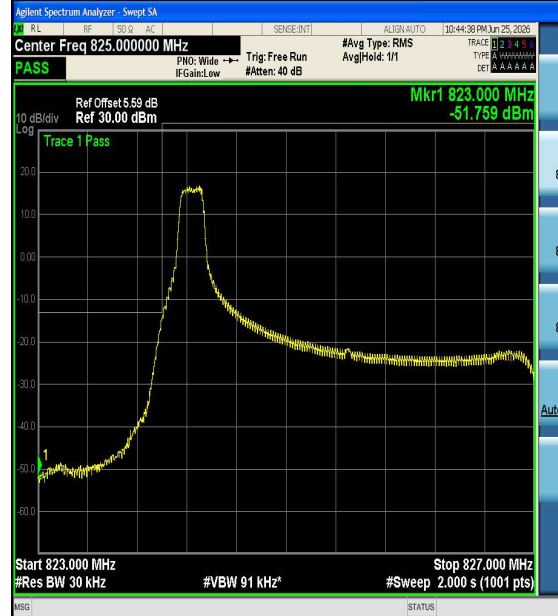
Band5-3MHz-16QAM-20415-1RB#0-PASS
