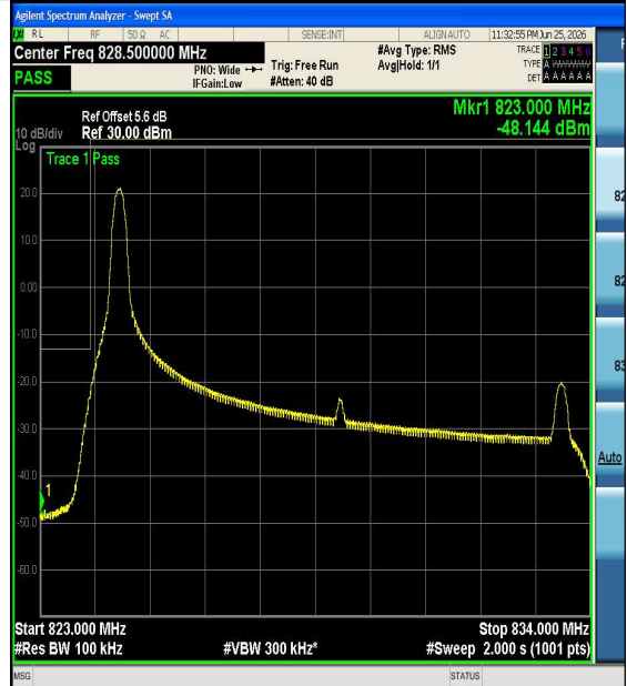
Band5-10MHz-16QAM-20450-1RB#0-PASS
