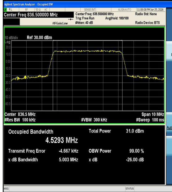
Band5-5MHz-16QAM-20525-25RB#0-PASS
