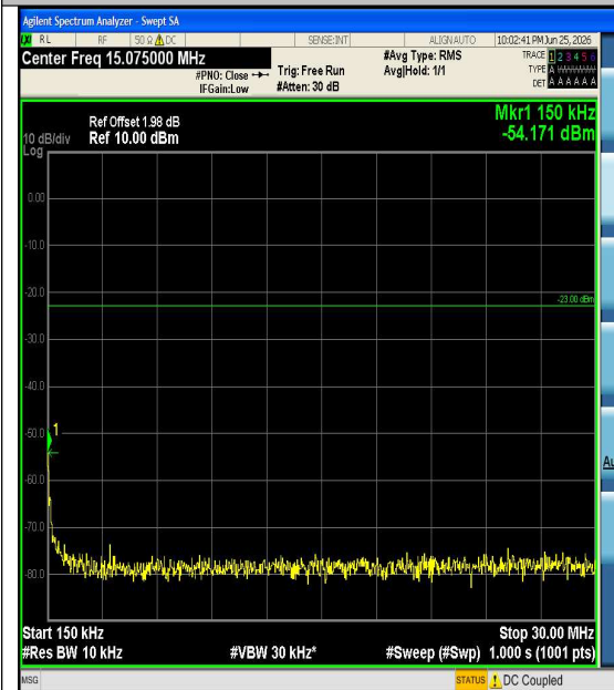
Band5-1.4MHz-16QAM-20407-1RB#0-0.15~30-PA SS
