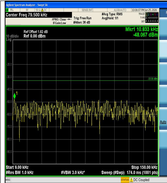
Band5-1.4MHz-QPSK-20643-1RB#0-0.009~0.15- PASS
