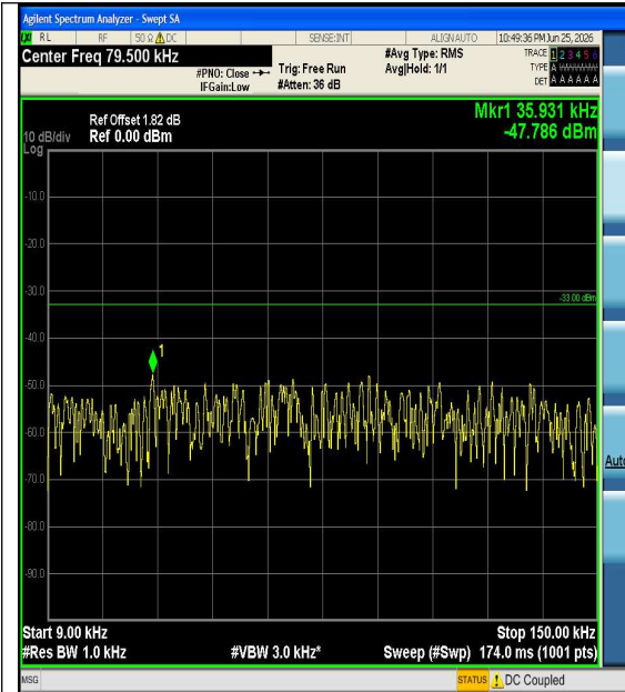
Band5-3MHz-QPSK-20525-1RB#0-0.009~0.15-PA SS
