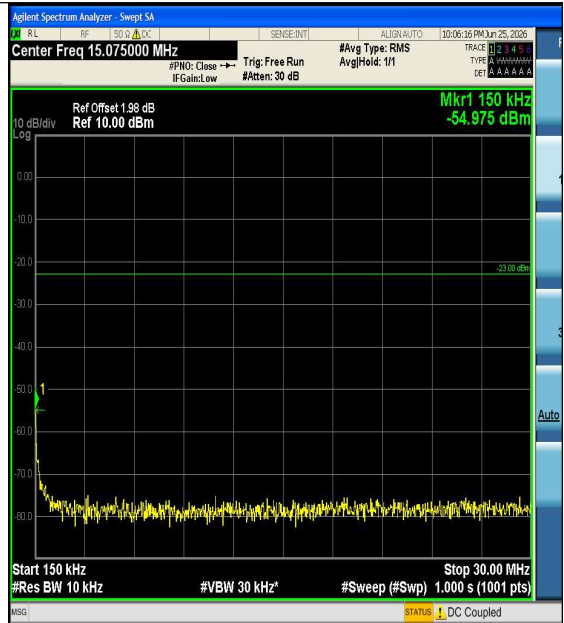
Band5-1.4MHz-QPSK-20643-1RB#0-0.15~30-PA SS
