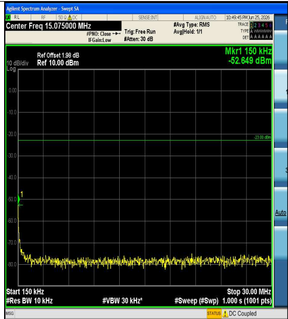
Band5-3MHz-QPSK-20525-1RB#0-0.15~30-PASS
