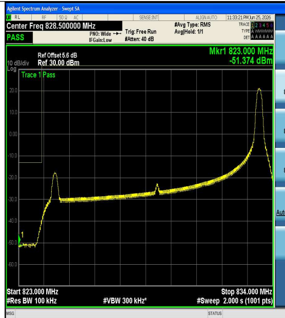
Band5-10MHz-16QAM-20450-1RB#49-PASS
