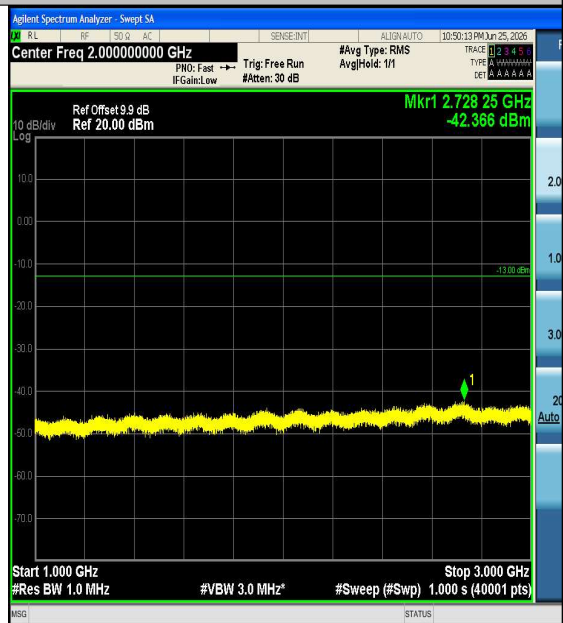
Band5-3MHz-QPSK-20525-1RB#0-1000~3000-PA SS
