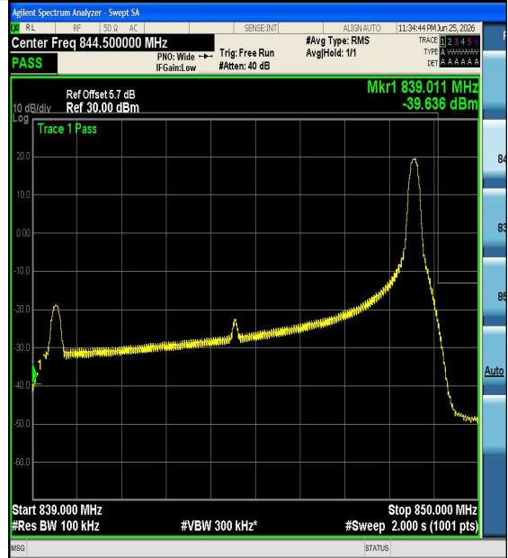
Band5-10MHz-16QAM-20600-1RB#49-PASS
