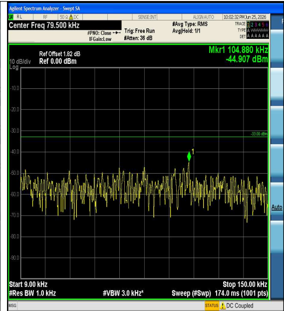
Band5-1.4MHz-16QAM-20407-1RB#0-0.009~0.15 -PASS
