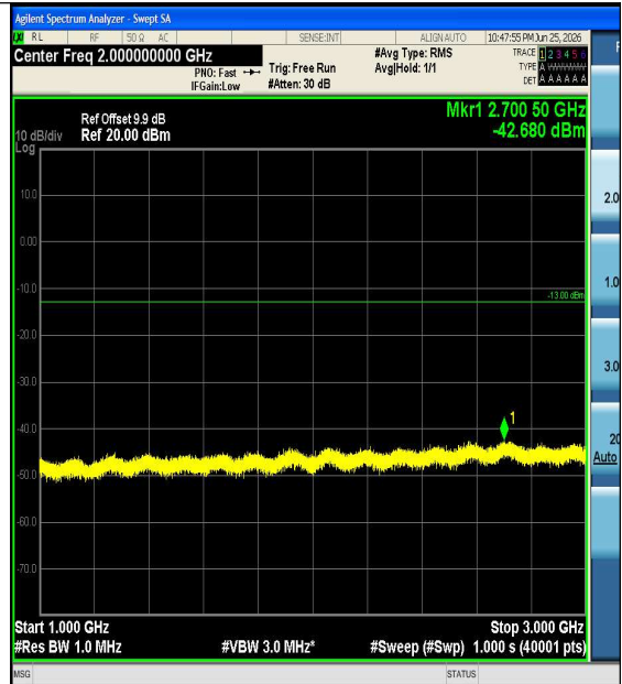
Band5-3MHz-QPSK-20415-1RB#0-1000~3000-PA
