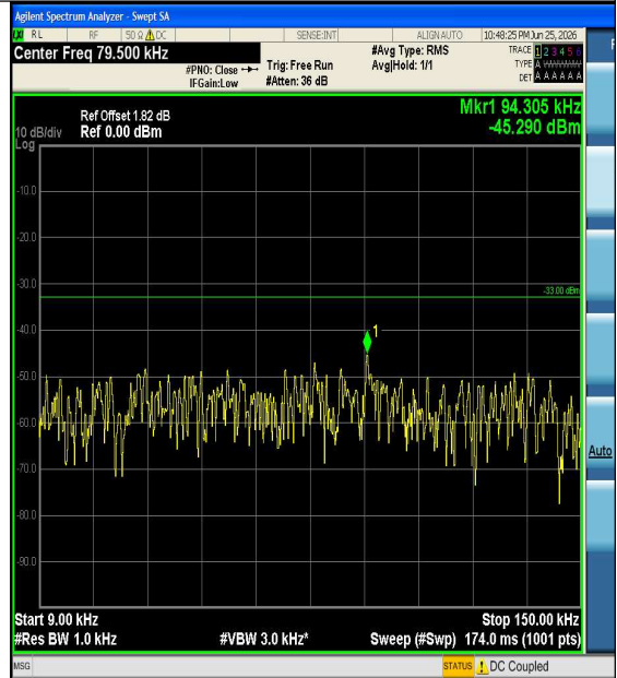
Band5-3MHz-16QAM-20415-1RB#0-0.009~0.15-P
