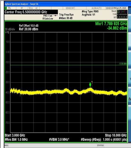
Band5-1.4MHz-QPSK-20407-1RB#0-3000~10000 -PASS
