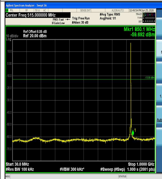
Band5-3MHz-QPSK-20525-1RB#0-30~1000-PAS S
