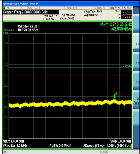
Band5-1.4MHz-QPSK-20643-1RB#0-1000~3000- PASS
