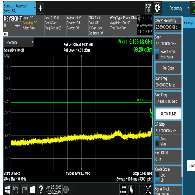
11AC40SISO-Ant1-5190-30~5140-PASS
