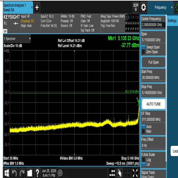
11N40SISO-Ant1-5190-30~5140-PASS
