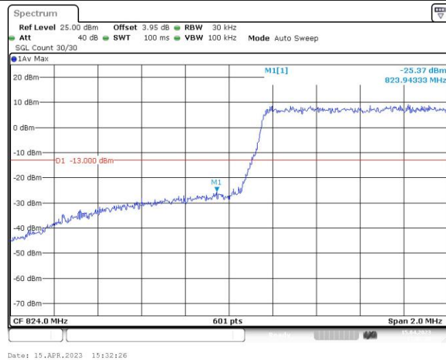
Band5-1.4MHz-16QAM-20643-1RB#0
