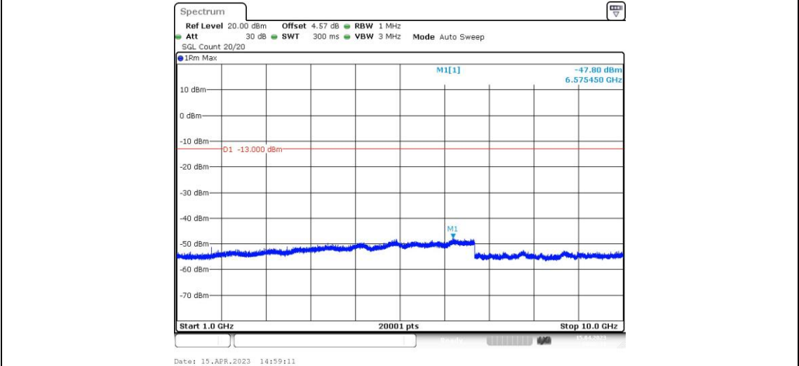
Band5-4233-4-1000~10000MHz
