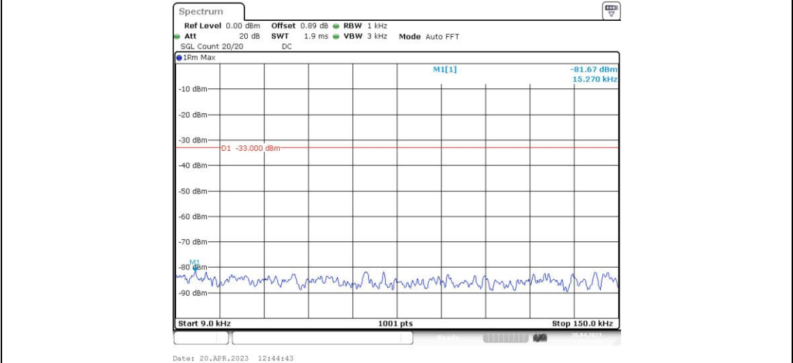
Band5-4233-2-0.009~0.15MHz
