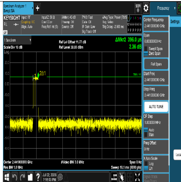
2DH1-Ant1-Hop-PASS
