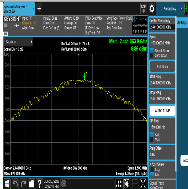
DH5-Ant1-2441-0~Reference-PASS
