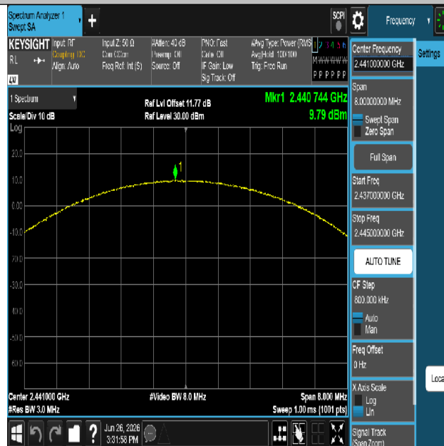
3DH5-Ant1-2441-PASS
