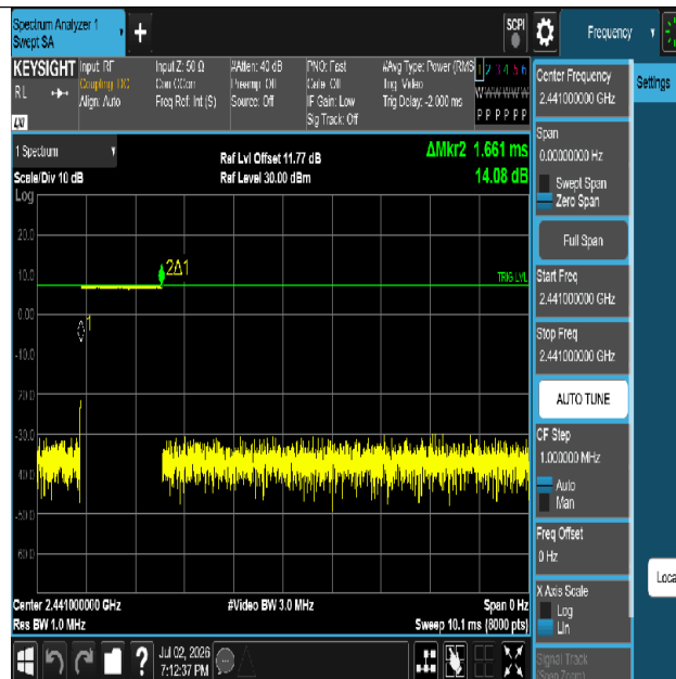
DH3-Ant1-Hop-PASS
