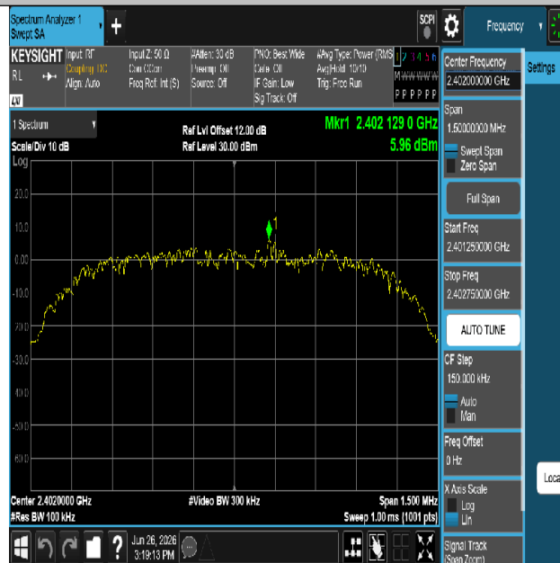
2DH5-Ant1-2402-0~Reference-PASS
