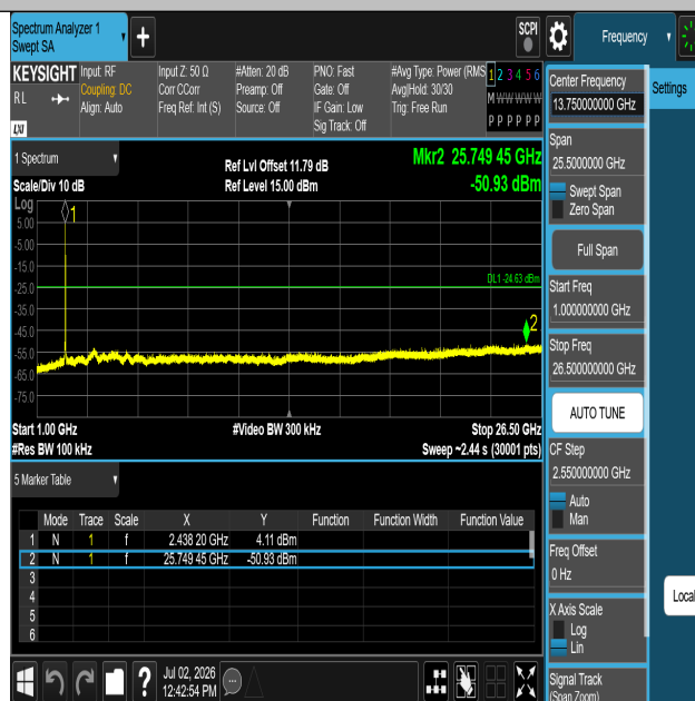
11B-Ant1-2437-1000~26500-PASS
