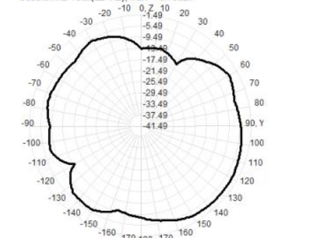
5850.0MHz Total(E2-YZ), Max= -3.70dBi
