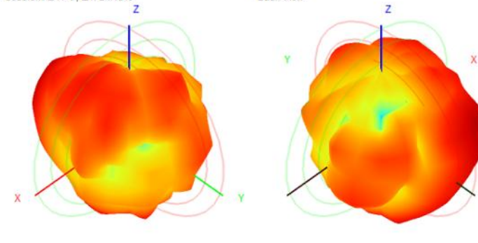
5850.0MHz H+V, Eff: 24.13%
