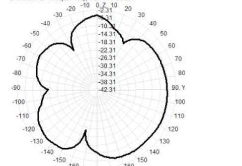
5850.0MHz Total(E2-YZ), Max= -3.70dBi
