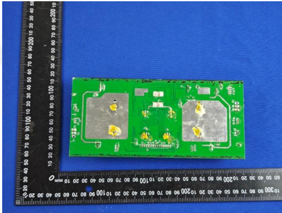
BP1032A2 BT&amp;BLE Antenna
